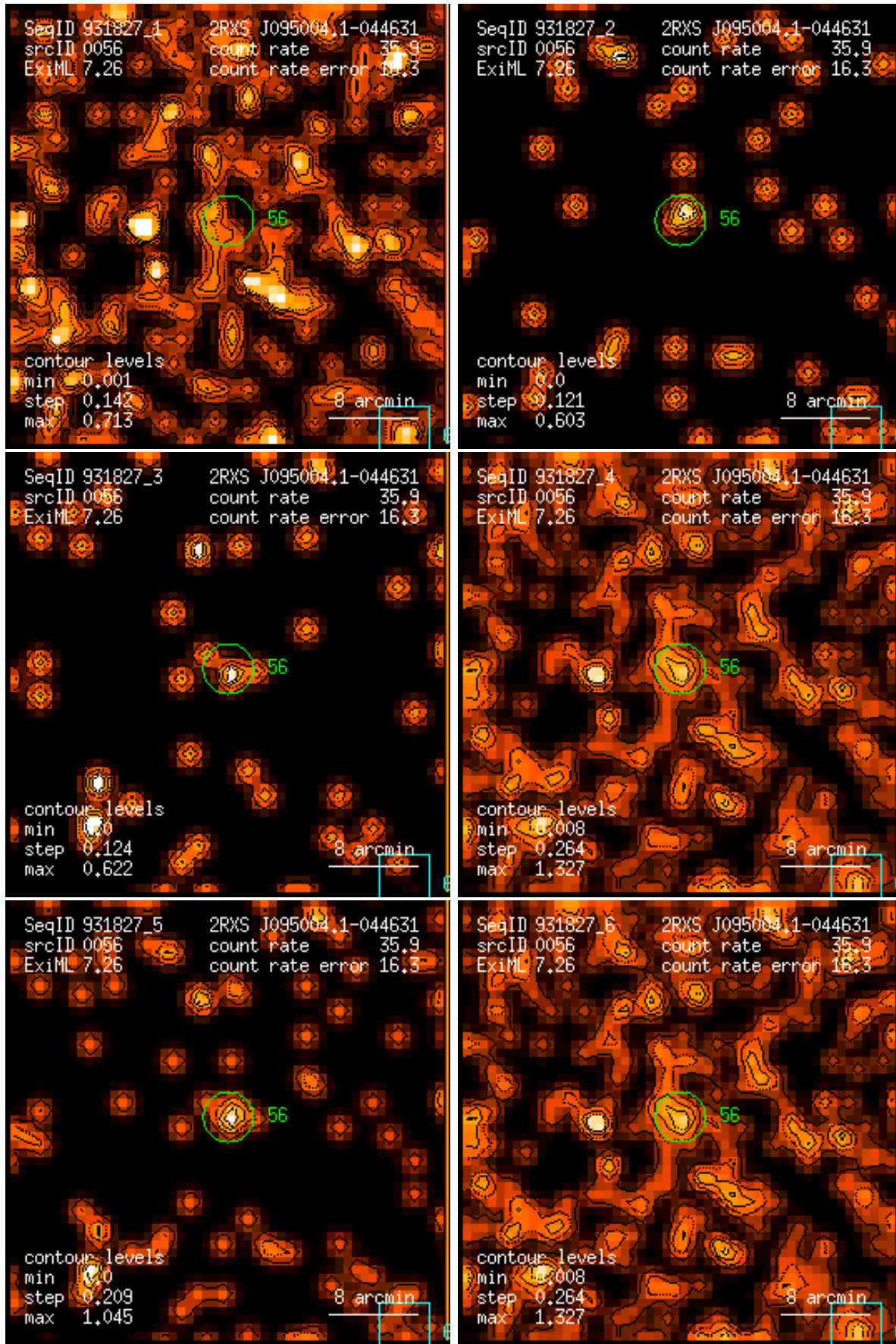
Figure 56: RASS 931827: detection 0056: band rate images, Gaussian filter: (1) PSPC channels 11 – 41, (2) 52 – 90, (3) 91 – 201, (4) 11 – 235, (5) 52 – 201, (6) 11 – 201. Broad band rates in counts/ks. Band rate contour levels in counts/ks/arcmin 2 .
