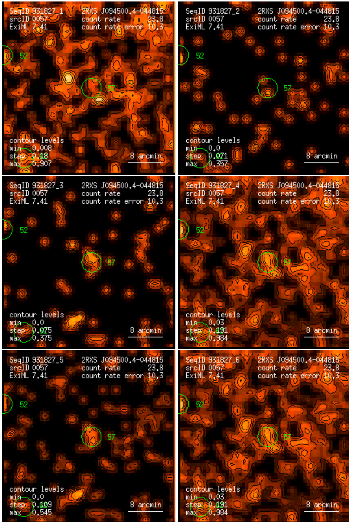
Figure 57: RASS 931827: detection 0057: band rate images, Gaussian filter: (1) PSPC channels 11 – 41, (2) 52 – 90, (3) 91 – 201, (4) 11 – 235, (5) 52 – 201, (6) 11 – 201. Broad band rates in counts/ks. Band rate contour levels in counts/ks/arcmin 2 .
