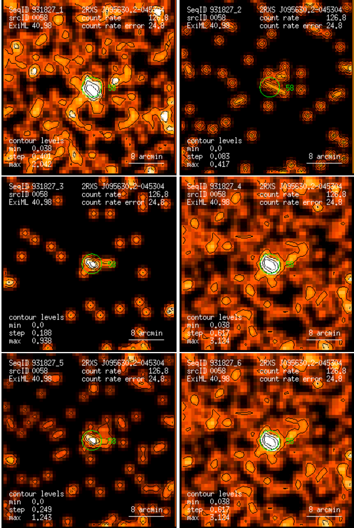
Figure 58: RASS 931827: detection 0058: band rate images, Gaussian filter: (1) PSPC channels 11 – 41, (2) 52 – 90, (3) 91 – 201, (4) 11 – 235, (5) 52 – 201, (6) 11 – 201. Broad band rates in counts/ks. Band rate contour levels in counts/ks/arcmin 2 .
