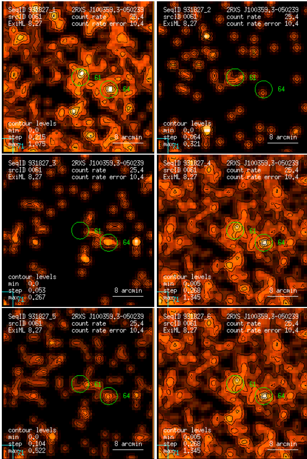
Figure 61: RASS 931827: detection 0061: band rate images, Gaussian filter: (1) PSPC channels 11 – 41, (2) 52 – 90, (3) 91 – 201, (4) 11 – 235, (5) 52 – 201, (6) 11 – 201. Broad band rates in counts/ks. Band rate contour levels in counts/ks/arcmin 2 .
