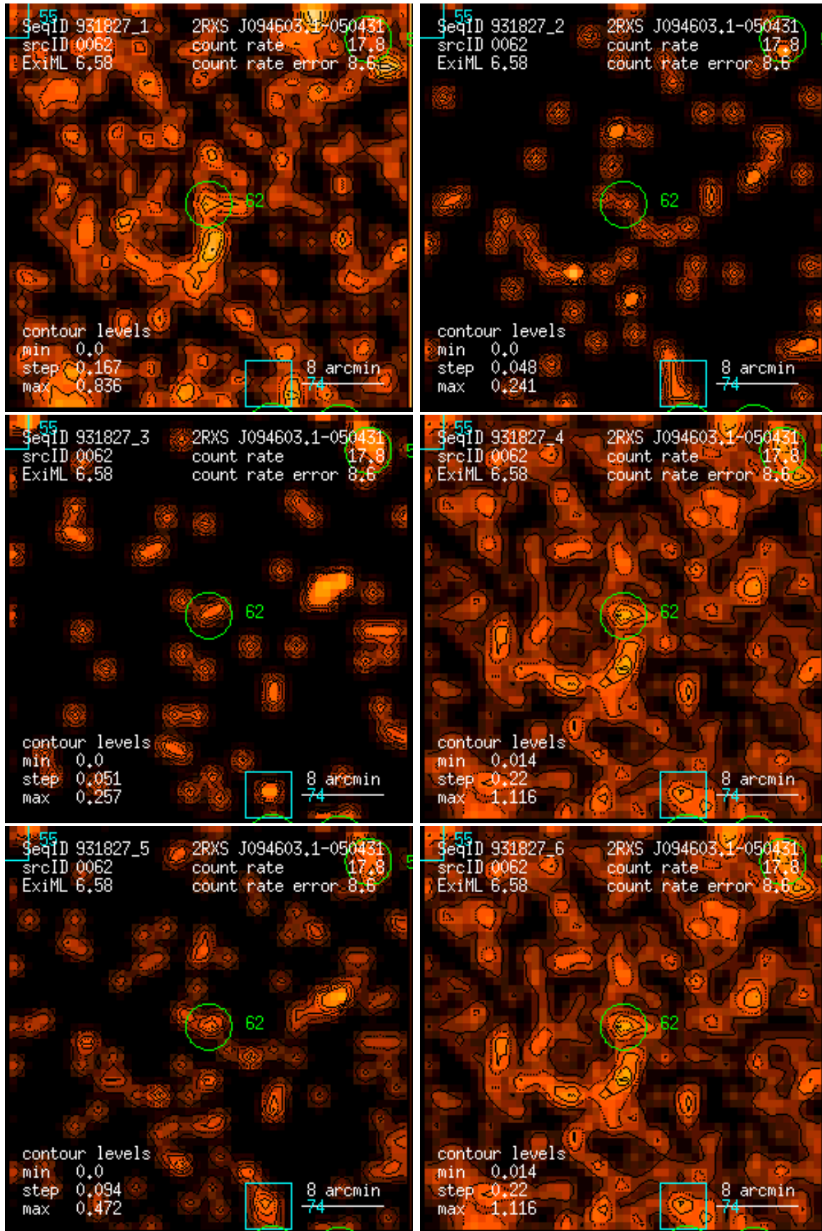
Figure 62: RASS 931827: detection 0062: band rate images, Gaussian filter: (1) PSPC channels 11 – 41, (2) 52 – 90, (3) 91 – 201, (4) 11 – 235, (5) 52 – 201, (6) 11 – 201. Broad band rates in counts/ks. Band rate contour levels in counts/ks/arcmin 2 .
