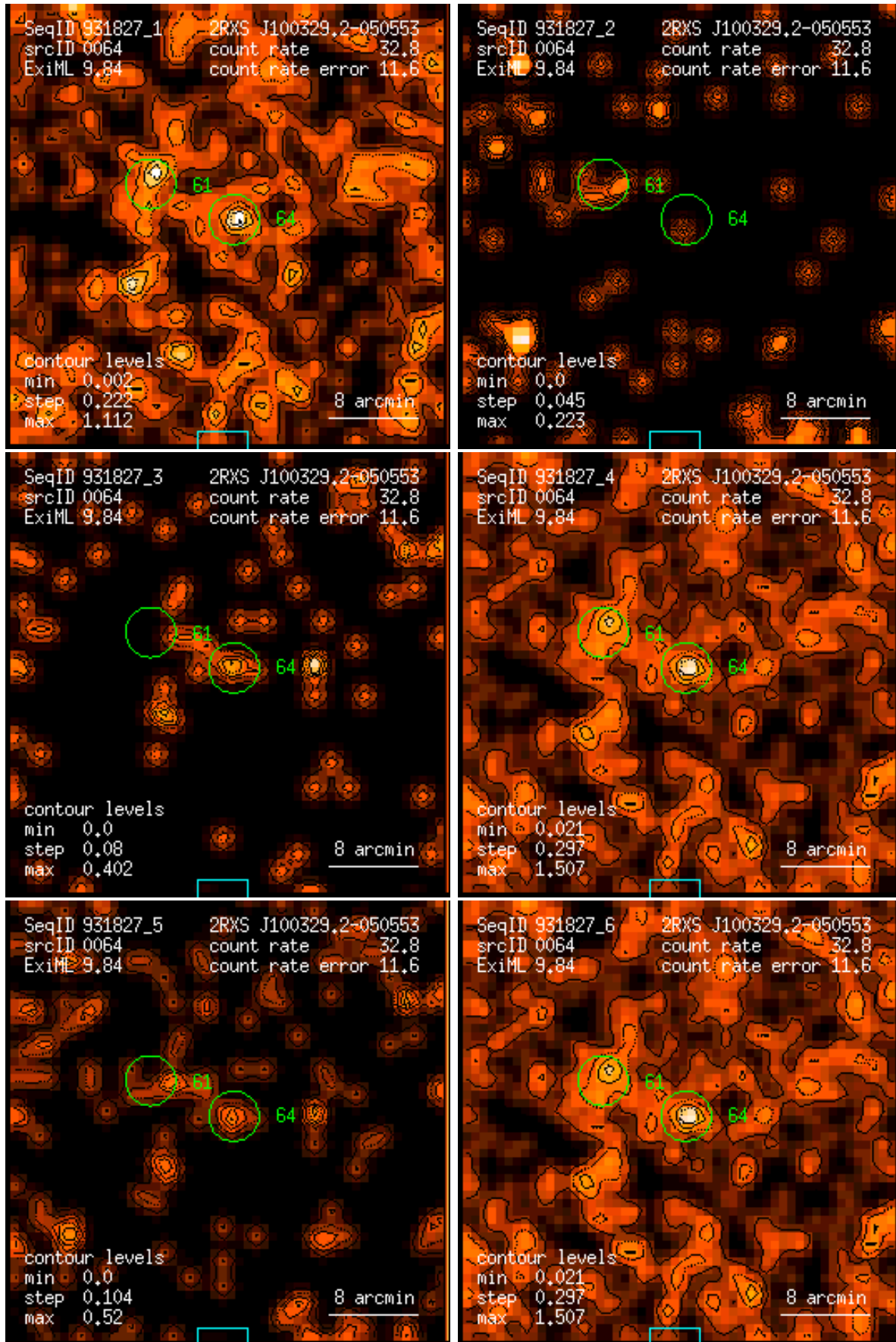
Figure 64: RASS 931827: detection 0064: band rate images, Gaussian filter: (1) PSPC channels 11 – 41, (2) 52 – 90, (3) 91 – 201, (4) 11 – 235, (5) 52 – 201, (6) 11 – 201. Broad band rates in counts/ks. Band rate contour levels in counts/ks/arcmin 2 .
