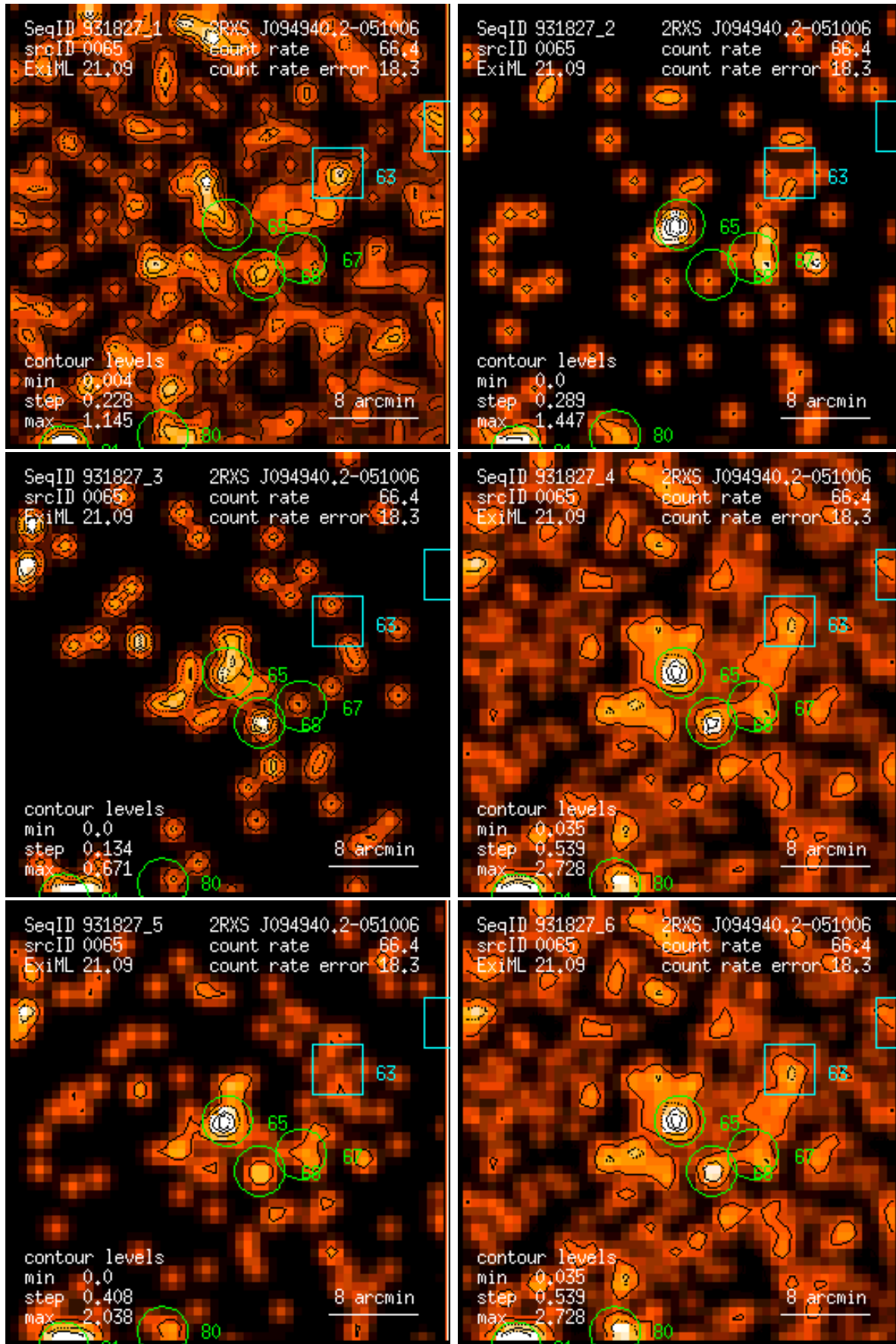
Figure 65: RASS 931827: detection 0065: band rate images, Gaussian filter: (1) PSPC channels 11 – 41, (2) 52 – 90, (3) 91 – 201, (4) 11 – 235, (5) 52 – 201, (6) 11 – 201. Broad band rates in counts/ks. Band rate contour levels in counts/ks/arcmin 2 .
