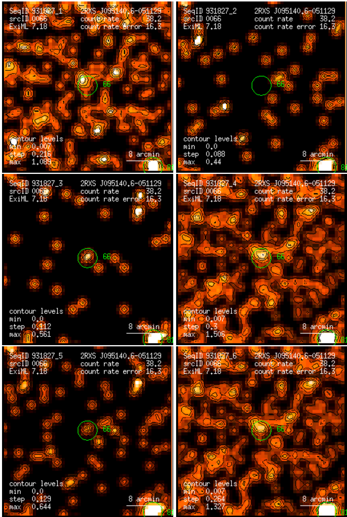
Figure 66: RASS 931827: detection 0066: band rate images, Gaussian filter: (1) PSPC channels 11 – 41, (2) 52 – 90, (3) 91 – 201, (4) 11 – 235, (5) 52 – 201, (6) 11 – 201. Broad band rates in counts/ks. Band rate contour levels in counts/ks/arcmin 2 .
