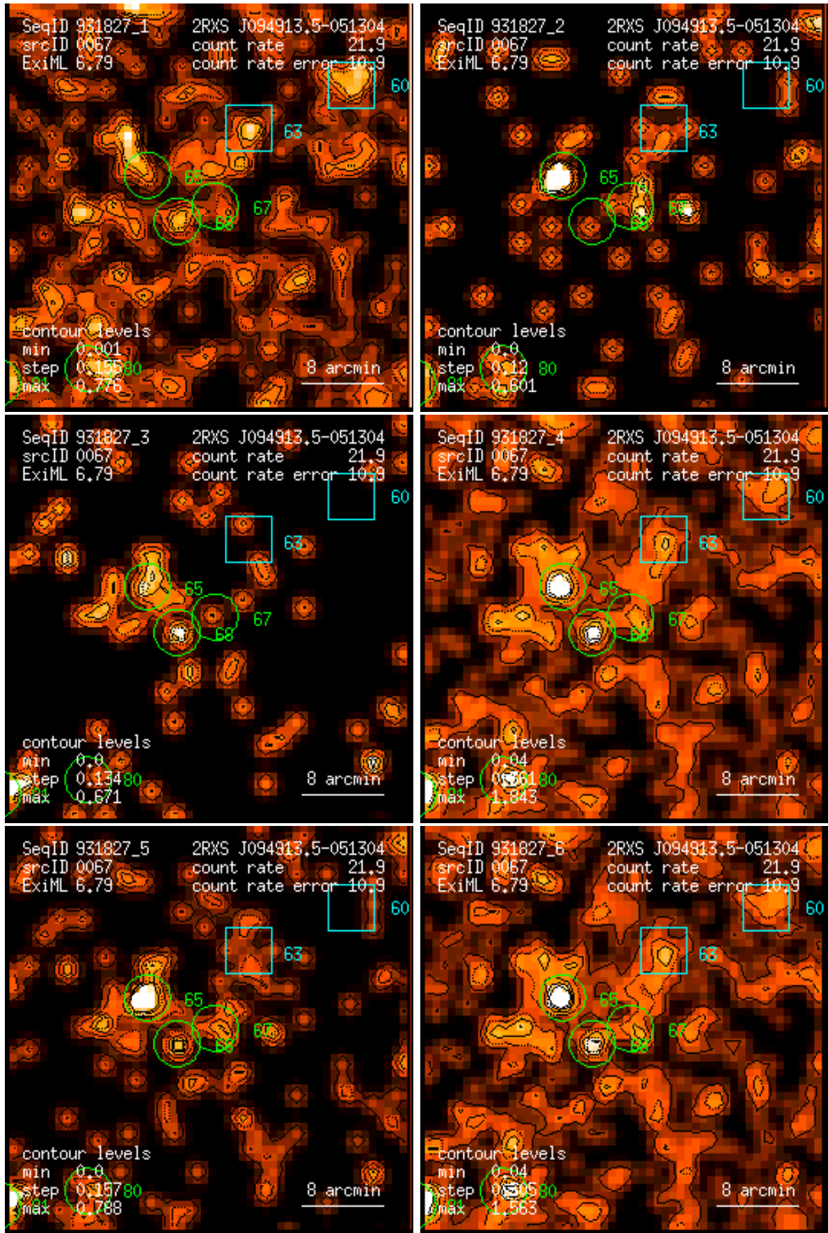
Figure 67: RASS 931827: detection 0067: band rate images, Gaussian filter: (1) PSPC channels 11 – 41, (2) 52 – 90, (3) 91 – 201, (4) 11 – 235, (5) 52 – 201, (6) 11 – 201. Broad band rates in counts/ks. Band rate contour levels in counts/ks/arcmin 2 .
