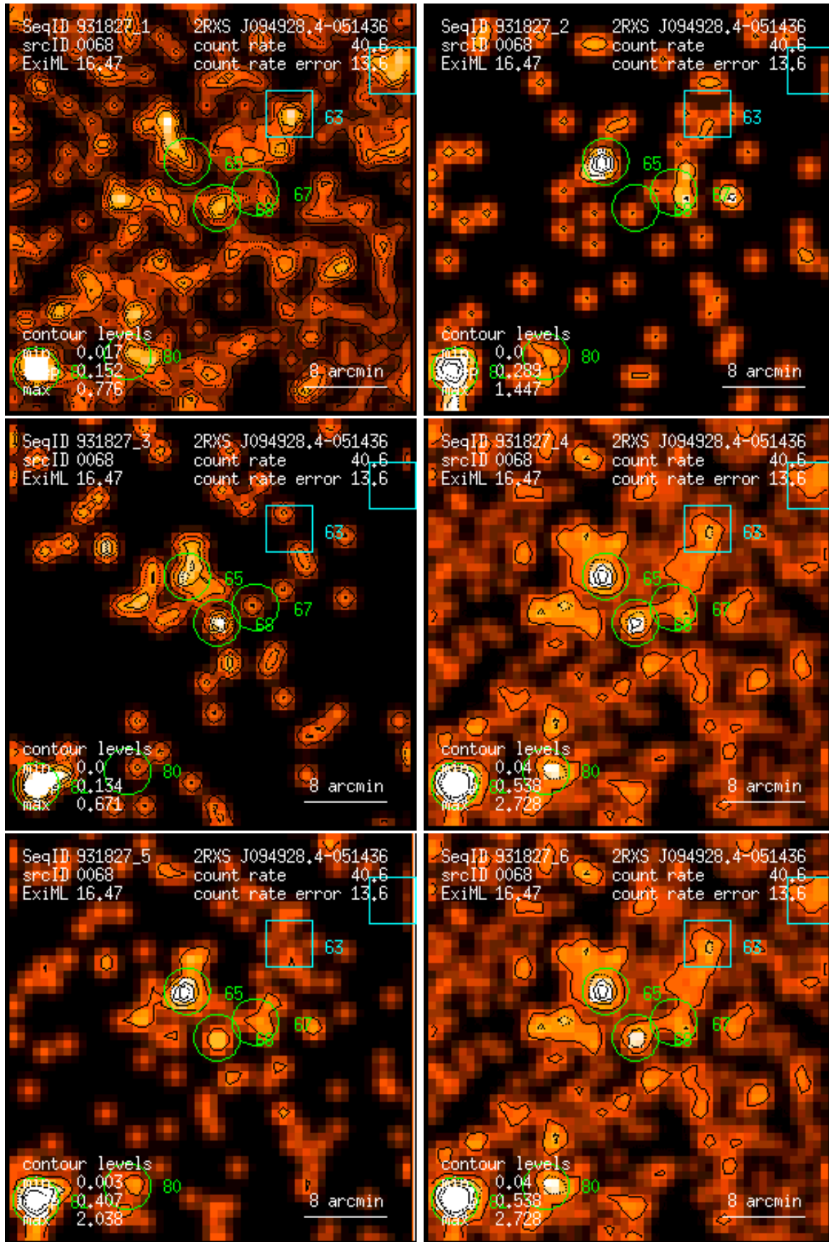
Figure 68: RASS 931827: detection 0068: band rate images, Gaussian filter: (1) PSPC channels 11 – 41, (2) 52 – 90, (3) 91 – 201, (4) 11 – 235, (5) 52 – 201, (6) 11 – 201. Broad band rates in counts/ks. Band rate contour levels in counts/ks/arcmin 2 .
