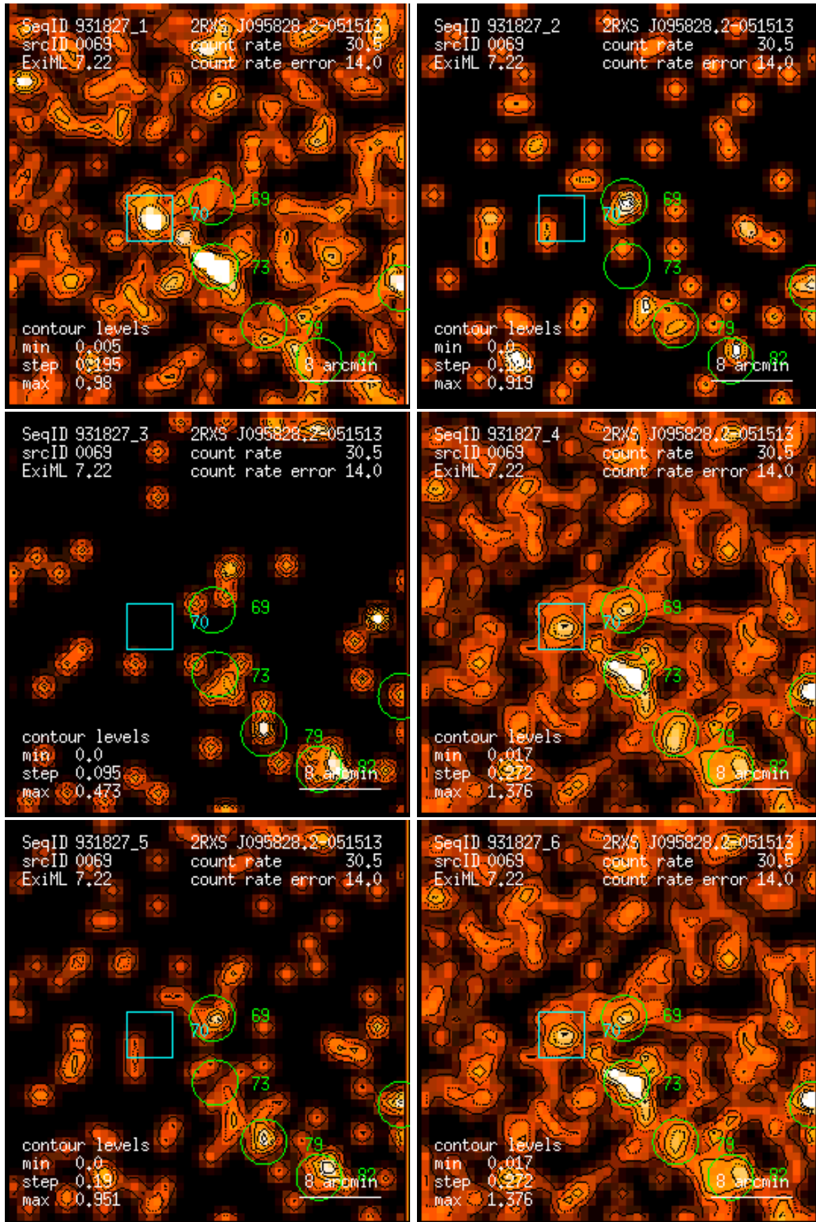
Figure 69: RASS 931827: detection 0069: band rate images, Gaussian filter: (1) PSPC channels 11 – 41, (2) 52 – 90, (3) 91 – 201, (4) 11 – 235, (5) 52 – 201, (6) 11 – 201. Broad band rates in counts/ks. Band rate contour levels in counts/ks/arcmin 2 .
