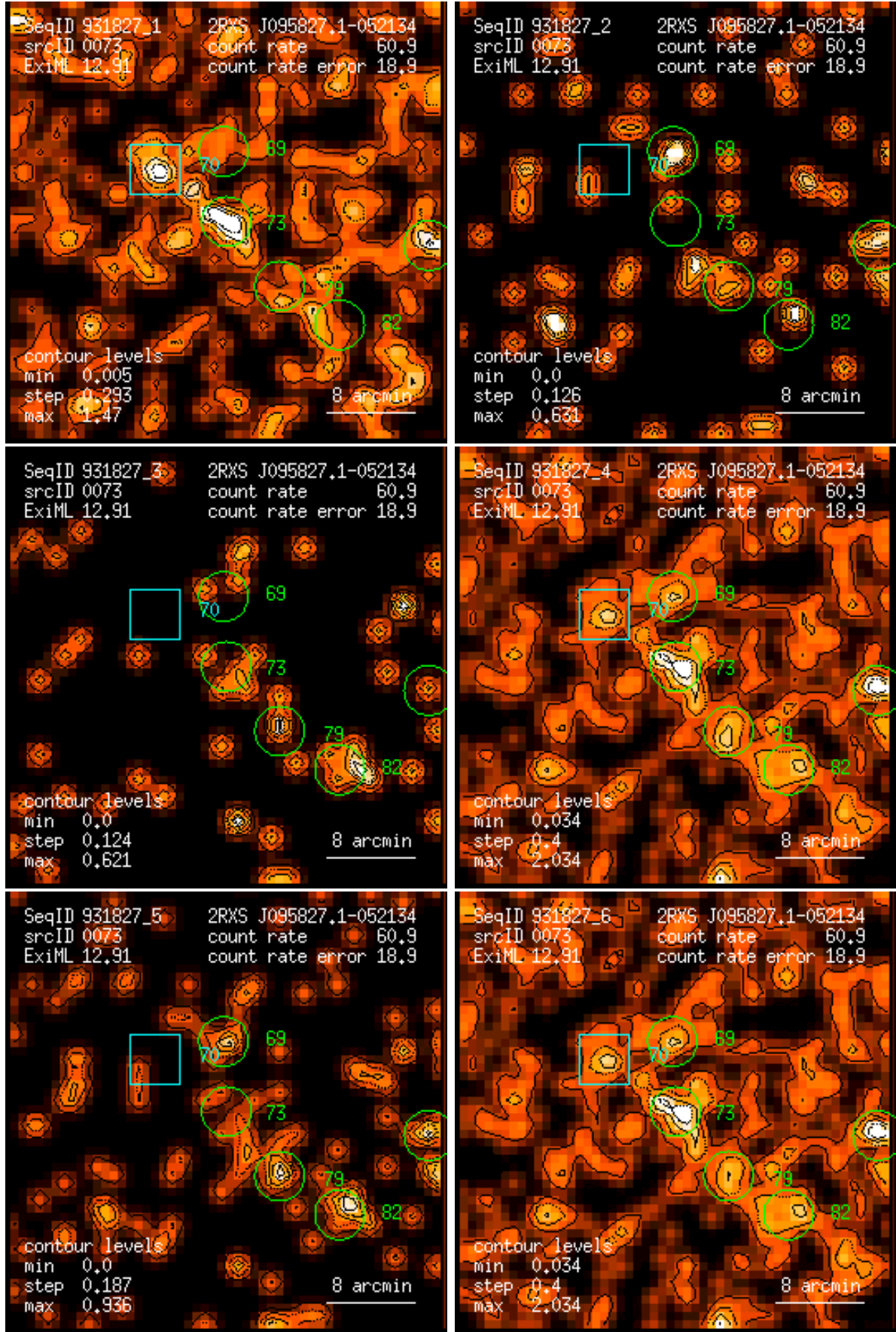
Figure 73: RASS 931827: detection 0073: band rate images, Gaussian filter: (1) PSPC channels 11 – 41, (2) 52 – 90, (3) 91 – 201, (4) 11 – 235, (5) 52 – 201, (6) 11 – 201. Broad band rates in counts/ks. Band rate contour levels in counts/ks/arcmin 2 .
