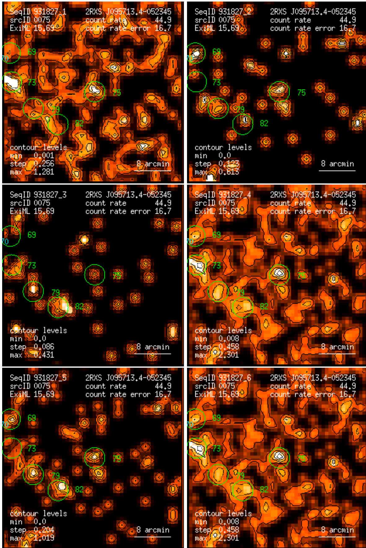
Figure 75: RASS 931827: detection 0075: band rate images, Gaussian filter: (1) PSPC channels 11 – 41, (2) 52 – 90, (3) 91 – 201, (4) 11 – 235, (5) 52 – 201, (6) 11 – 201. Broad band rates in counts/ks. Band rate contour levels in counts/ks/arcmin 2 .
