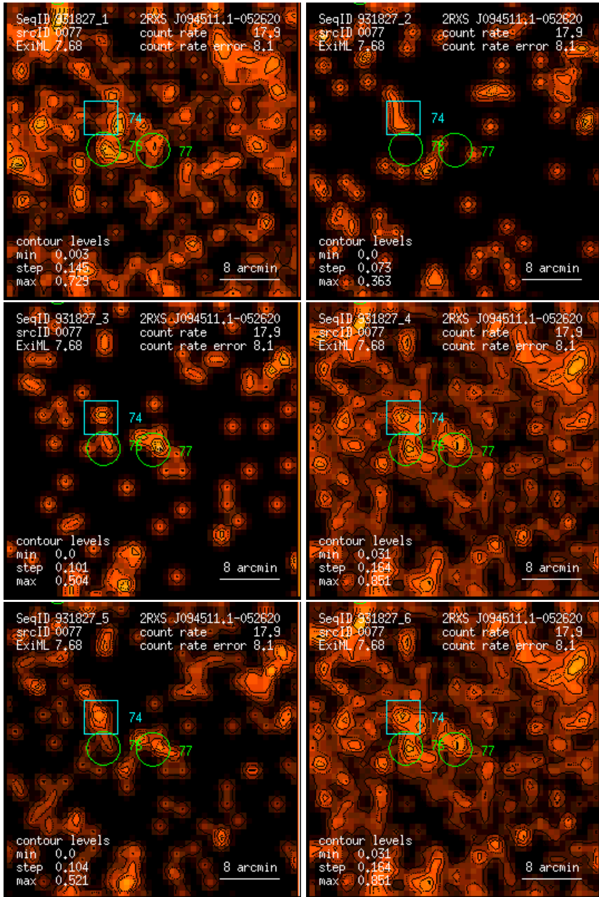
Figure 77: RASS 931827: detection 0077: band rate images, Gaussian filter: (1) PSPC channels 11 – 41, (2) 52 – 90, (3) 91 – 201, (4) 11 – 235, (5) 52 – 201, (6) 11 – 201. Broad band rates in counts/ks. Band rate contour levels in counts/ks/arcmin 2 .
