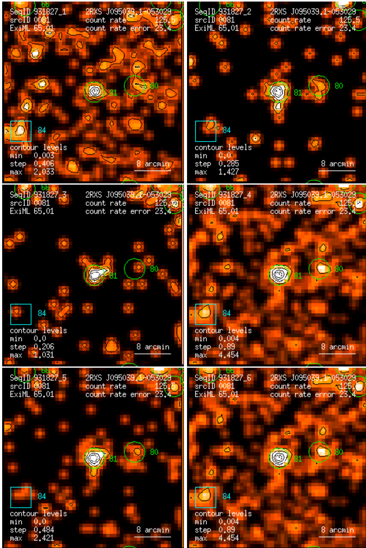
Figure 81: RASS 931827: detection 0081: band rate images, Gaussian filter: (1) PSPC channels 11 – 41, (2) 52 – 90, (3) 91 – 201, (4) 11 – 235, (5) 52 – 201, (6) 11 – 201. Broad band rates in counts/ks. Band rate contour levels in counts/ks/arcmin 2 .
