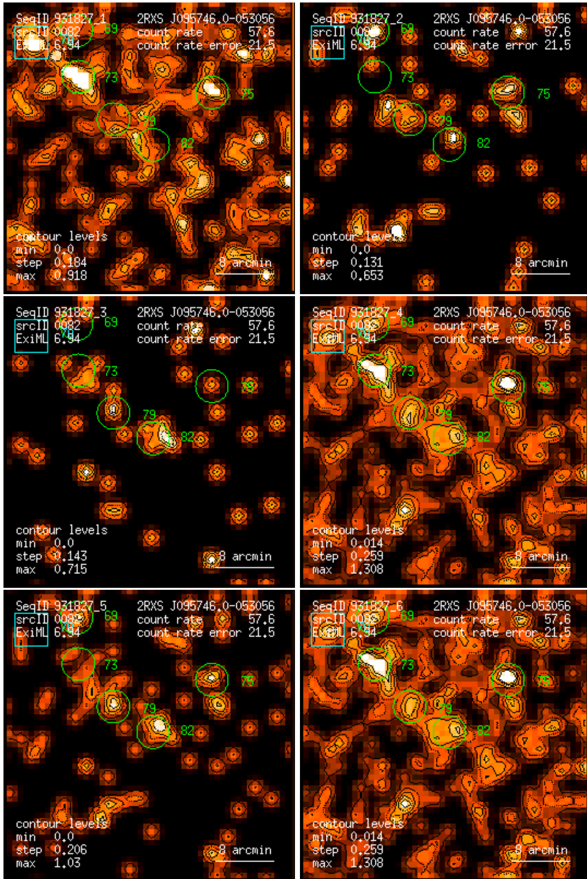
Figure 82: RASS 931827: detection 0082: band rate images, Gaussian filter: (1) PSPC channels 11 – 41, (2) 52 – 90, (3) 91 – 201, (4) 11 – 235, (5) 52 – 201, (6) 11 – 201. Broad band rates in counts/ks. Band rate contour levels in counts/ks/arcmin 2 .
