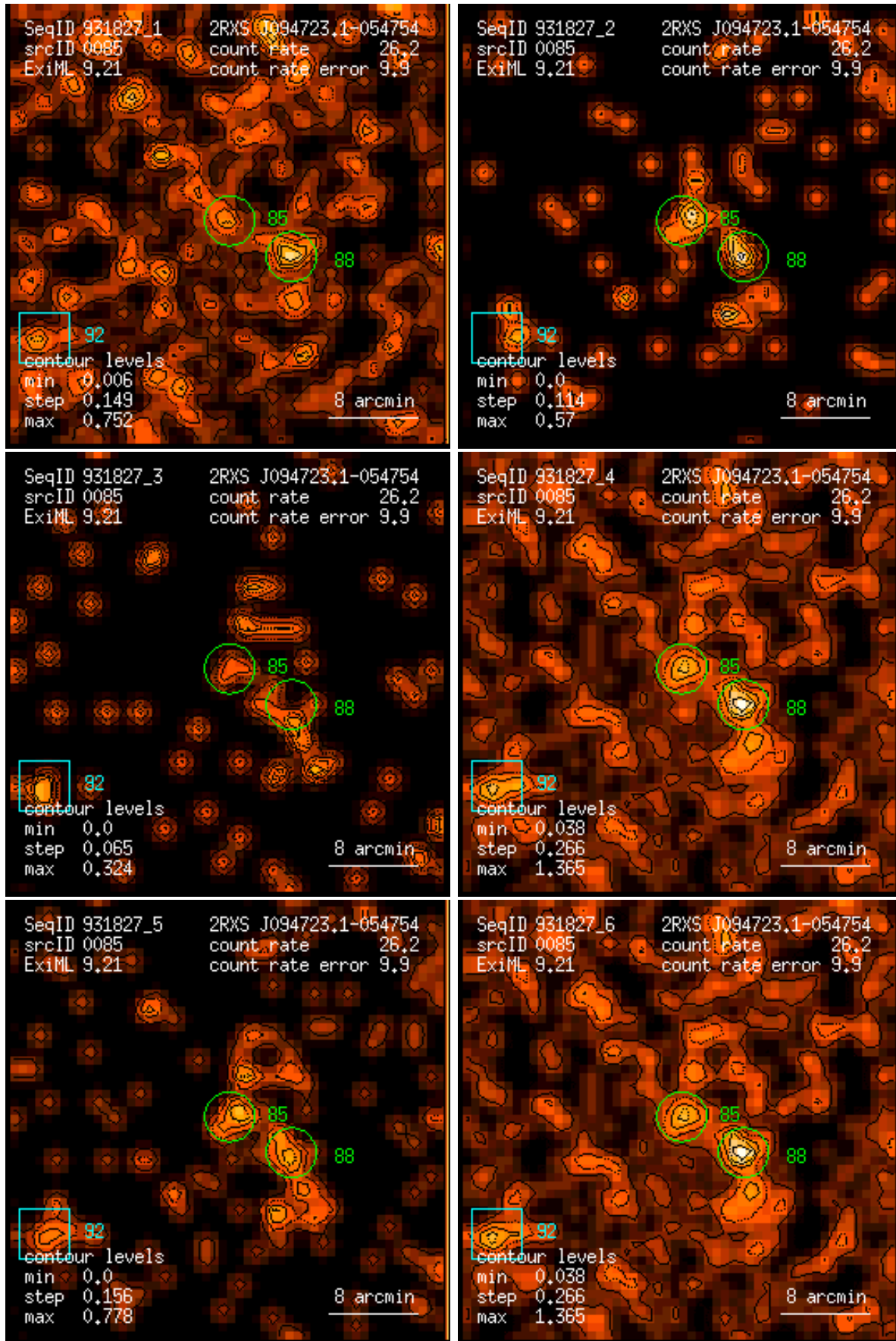
Figure 85: RASS 931827: detection 0085: band rate images, Gaussian filter: (1) PSPC channels 11 – 41, (2) 52 – 90, (3) 91 – 201, (4) 11 – 235, (5) 52 – 201, (6) 11 – 201. Broad band rates in counts/ks. Band rate contour levels in counts/ks/arcmin 2 .
