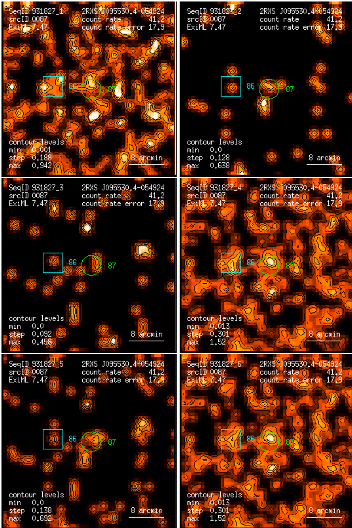
Figure 87: RASS 931827: detection 0087: band rate images, Gaussian filter: (1) PSPC channels 11 – 41, (2) 52 – 90, (3) 91 – 201, (4) 11 – 235, (5) 52 – 201, (6) 11 – 201. Broad band rates in counts/ks. Band rate contour levels in counts/ks/arcmin 2 .
