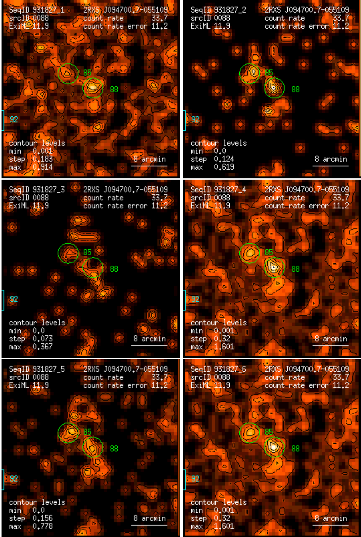
Figure 88: RASS 931827: detection 0088: band rate images, Gaussian filter: (1) PSPC channels 11 – 41, (2) 52 – 90, (3) 91 – 201, (4) 11 – 235, (5) 52 – 201, (6) 11 – 201. Broad band rates in counts/ks. Band rate contour levels in counts/ks/arcmin 2 .
