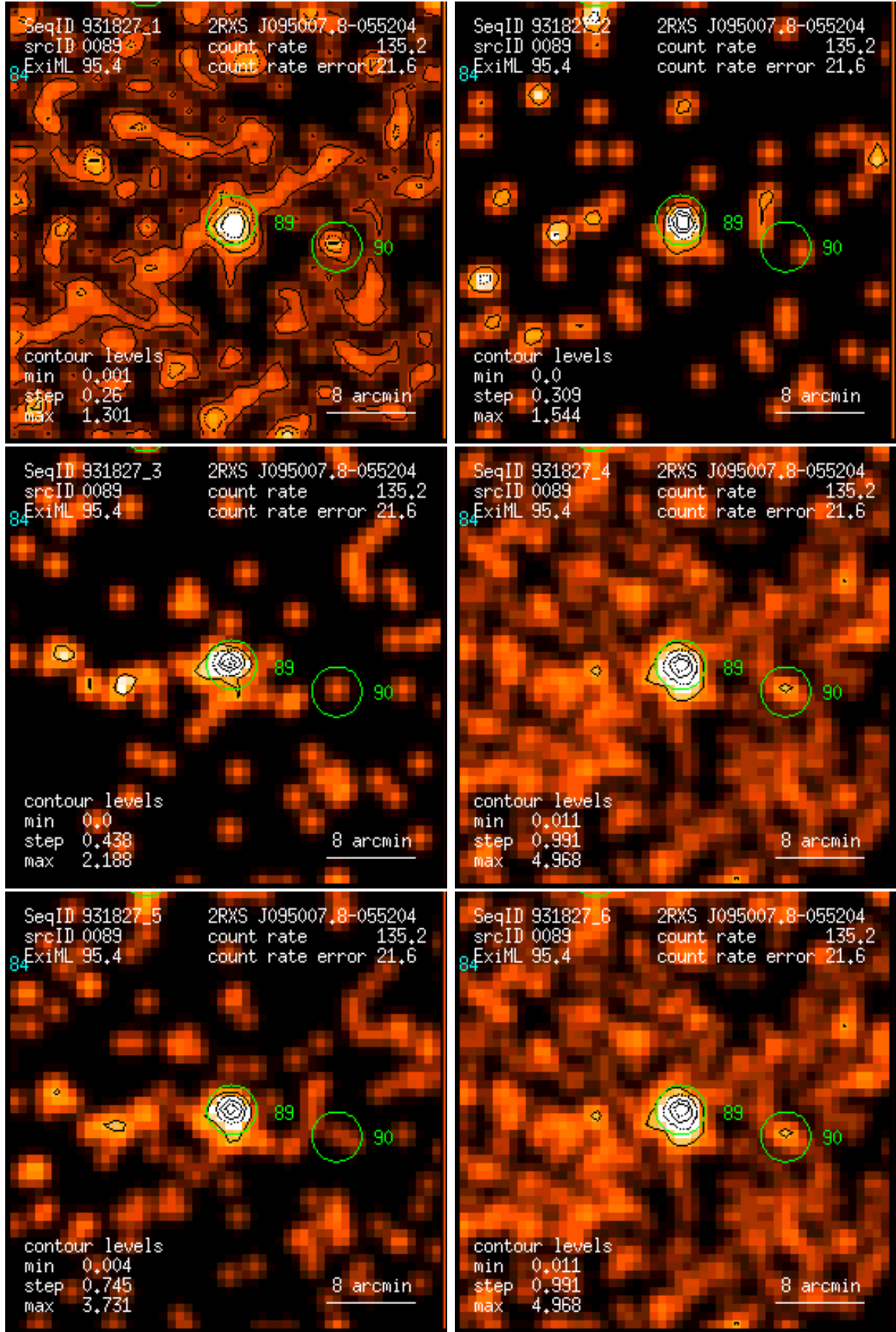
Figure 89: RASS 931827: detection 0089: band rate images, Gaussian filter: (1) PSPC channels 11 – 41, (2) 52 – 90, (3) 91 – 201, (4) 11 – 235, (5) 52 – 201, (6) 11 – 201. Broad band rates in counts/ks. Band rate contour levels in counts/ks/arcmin 2 .
