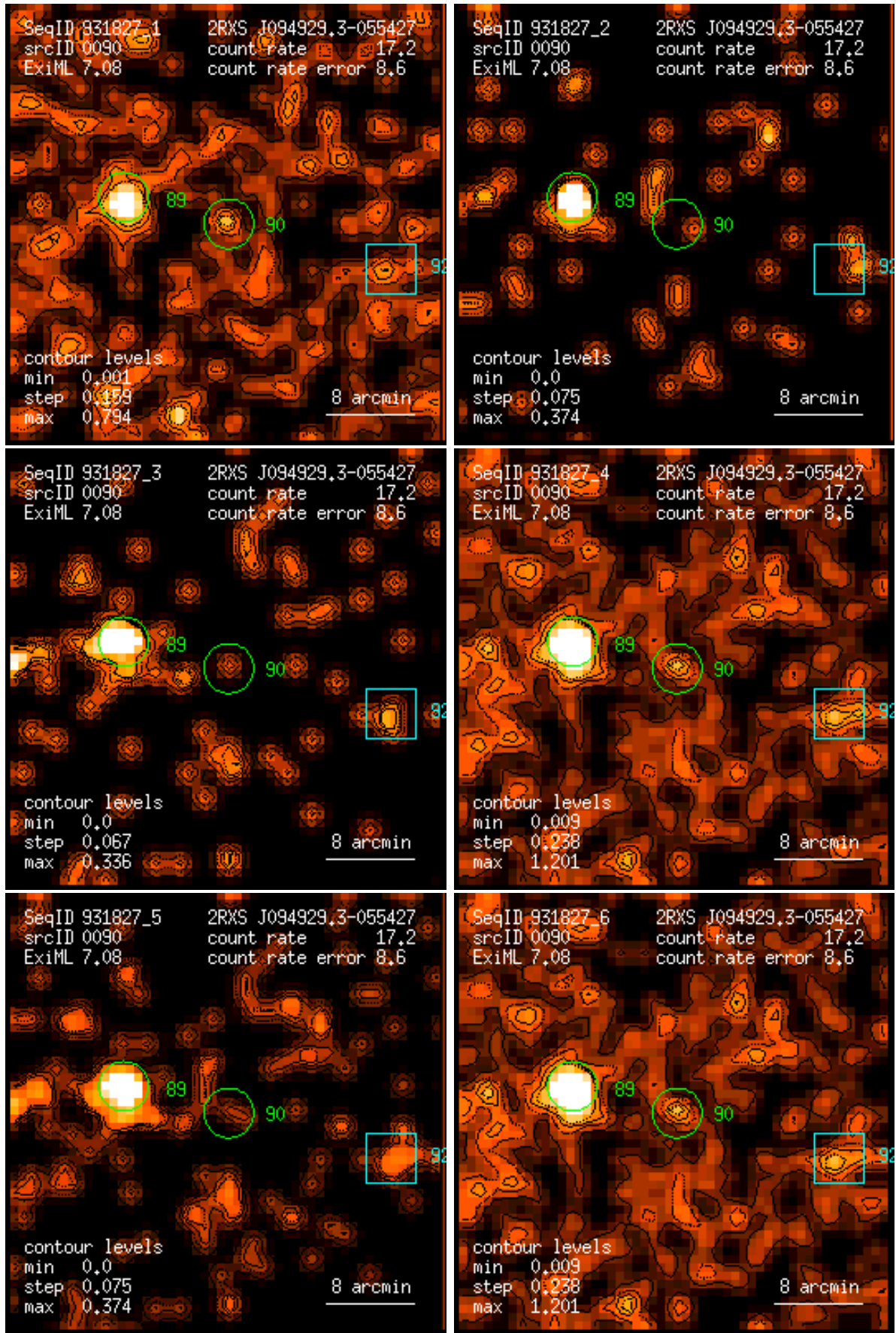
Figure 90: RASS 931827: detection 0090: band rate images, Gaussian filter: (1) PSPC channels 11 – 41, (2) 52 – 90, (3) 91 – 201, (4) 11 – 235, (5) 52 – 201, (6) 11 – 201. Broad band rates in counts/ks. Band rate contour levels in counts/ks/arcmin 2 .
