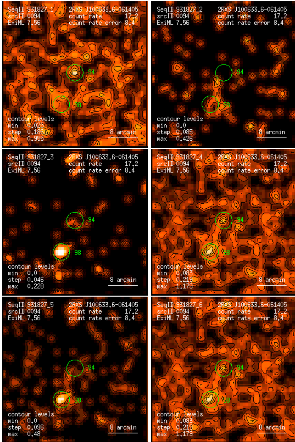
Figure 94: RASS 931827: detection 0094: band rate images, Gaussian filter: (1) PSPC channels 11 – 41, (2) 52 – 90, (3) 91 – 201, (4) 11 – 235, (5) 52 – 201, (6) 11 – 201. Broad band rates in counts/ks. Band rate contour levels in counts/ks/arcmin 2 .
