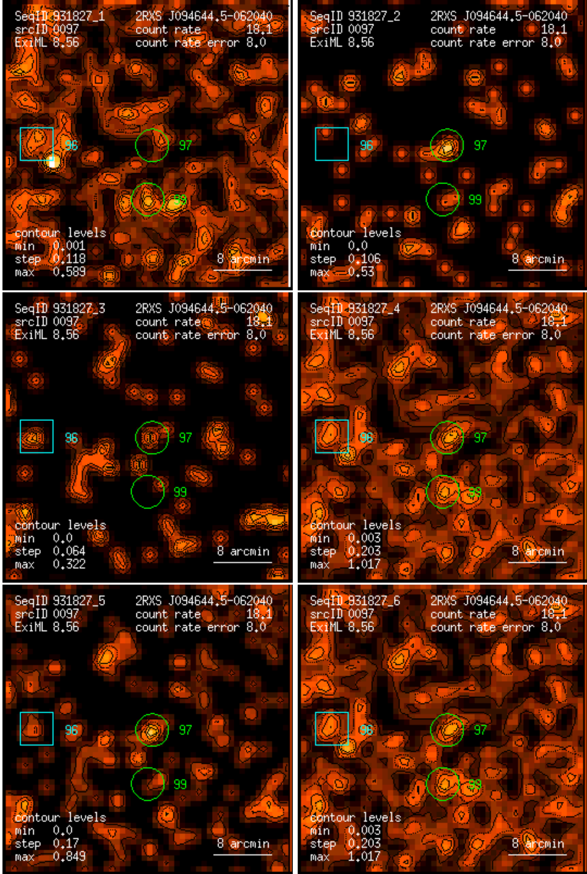
Figure 97: RASS 931827: detection 0097: band rate images, Gaussian filter: (1) PSPC channels 11 – 41, (2) 52 – 90, (3) 91 – 201, (4) 11 – 235, (5) 52 – 201, (6) 11 – 201. Broad band rates in counts/ks. Band rate contour levels in counts/ks/arcmin 2 .
