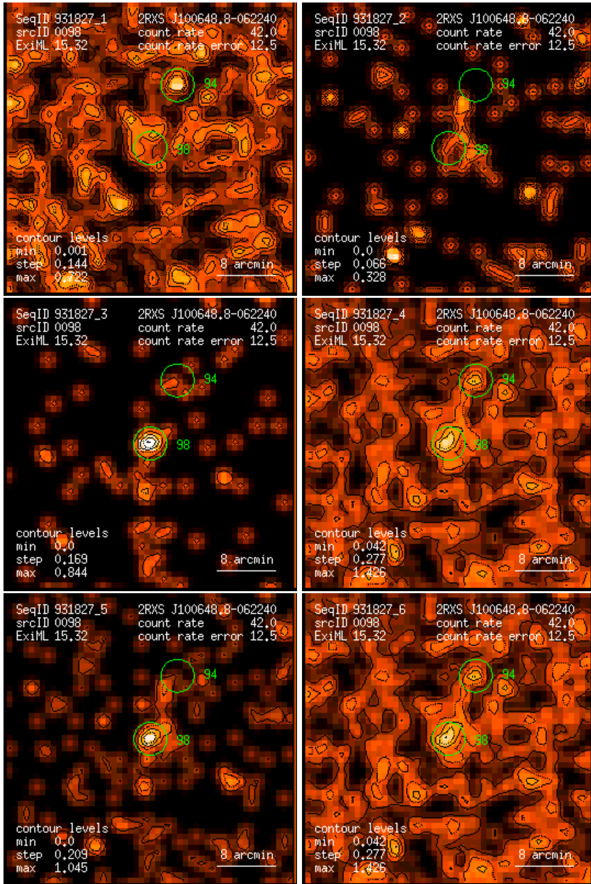
Figure 98: RASS 931827: detection 0098: band rate images, Gaussian filter: (1) PSPC channels 11 – 41, (2) 52 – 90, (3) 91 – 201, (4) 11 – 235, (5) 52 – 201, (6) 11 – 201. Broad band rates in counts/ks. Band rate contour levels in counts/ks/arcmin 2 .
