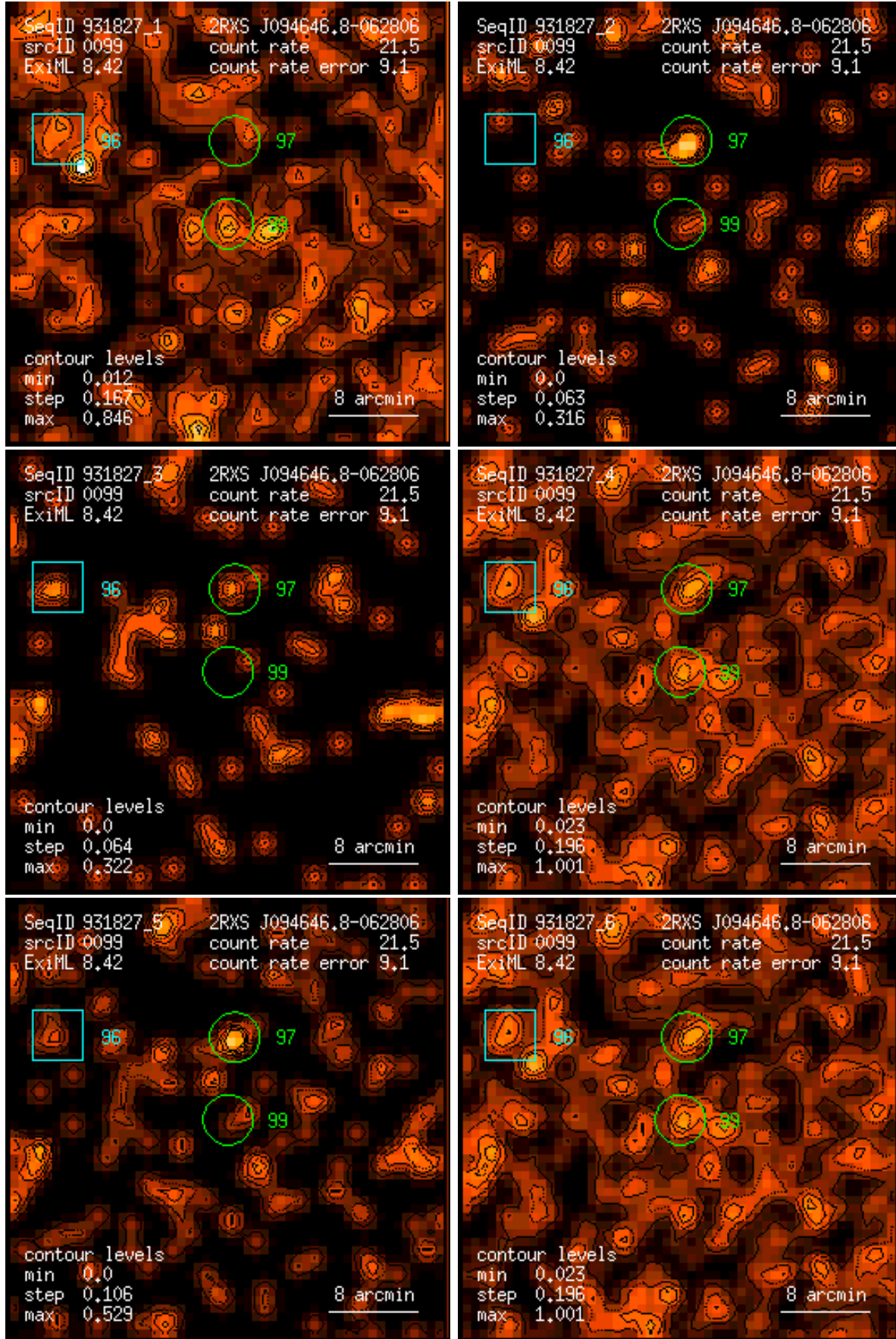
Figure 99: RASS 931827: detection 0099: band rate images, Gaussian filter: (1) PSPC channels 11 – 41, (2) 52 – 90, (3) 91 – 201, (4) 11 – 235, (5) 52 – 201, (6) 11 – 201. Broad band rates in counts/ks. Band rate contour levels in counts/ks/arcmin 2 .
