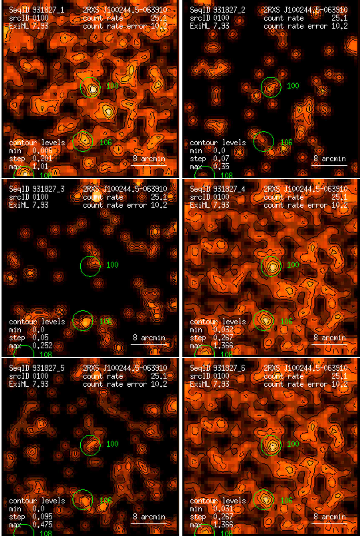
Figure 100: RASS 931827: detection 0100: band rate images, Gaussian filter: (1) PSPC channels 11 – 41, (2) 52 – 90, (3) 91 – 201, (4) 11 – 235, (5) 52 – 201, (6) 11 – 201. Broad band rates in counts/ks. Band rate contour levels in counts/ks/arcmin 2 .
