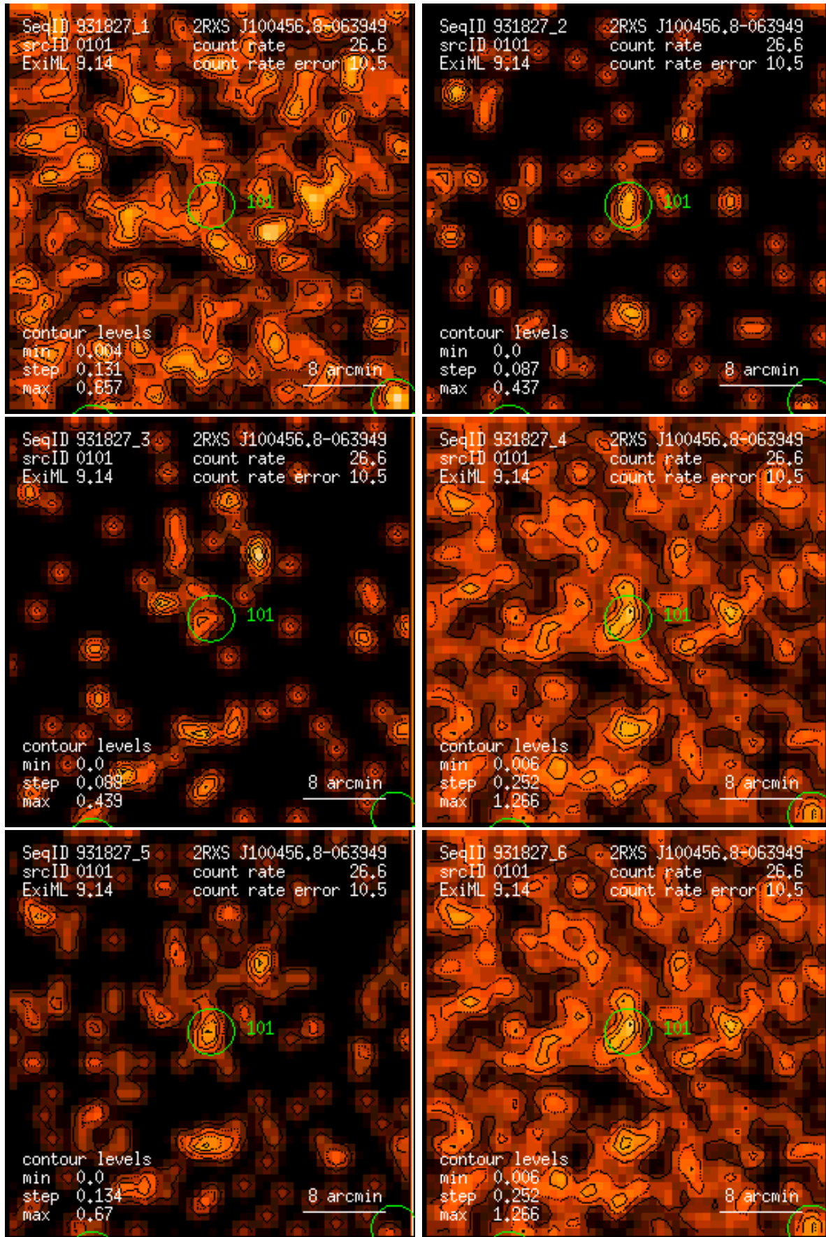
Figure 101: RASS 931827: detection 0101: band rate images, Gaussian filter: (1) PSPC channels 11 – 41, (2) 52 – 90, (3) 91 – 201, (4) 11 – 235, (5) 52 – 201, (6) 11 – 201. Broad band rates in counts/ks. Band rate contour levels in counts/ks/arcmin 2 .
