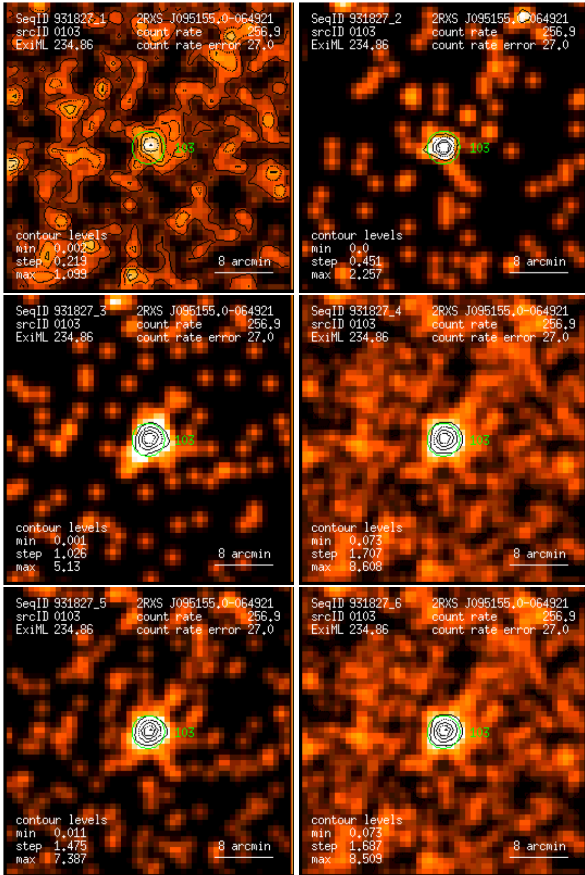
Figure 103: RASS 931827: detection 0103: band rate images, Gaussian filter: (1) PSPC channels 11 – 41, (2) 52 – 90, (3) 91 – 201, (4) 11 – 235, (5) 52 – 201, (6) 11 – 201. Broad band rates in counts/ks. Band rate contour levels in counts/ks/arcmin 2 .
