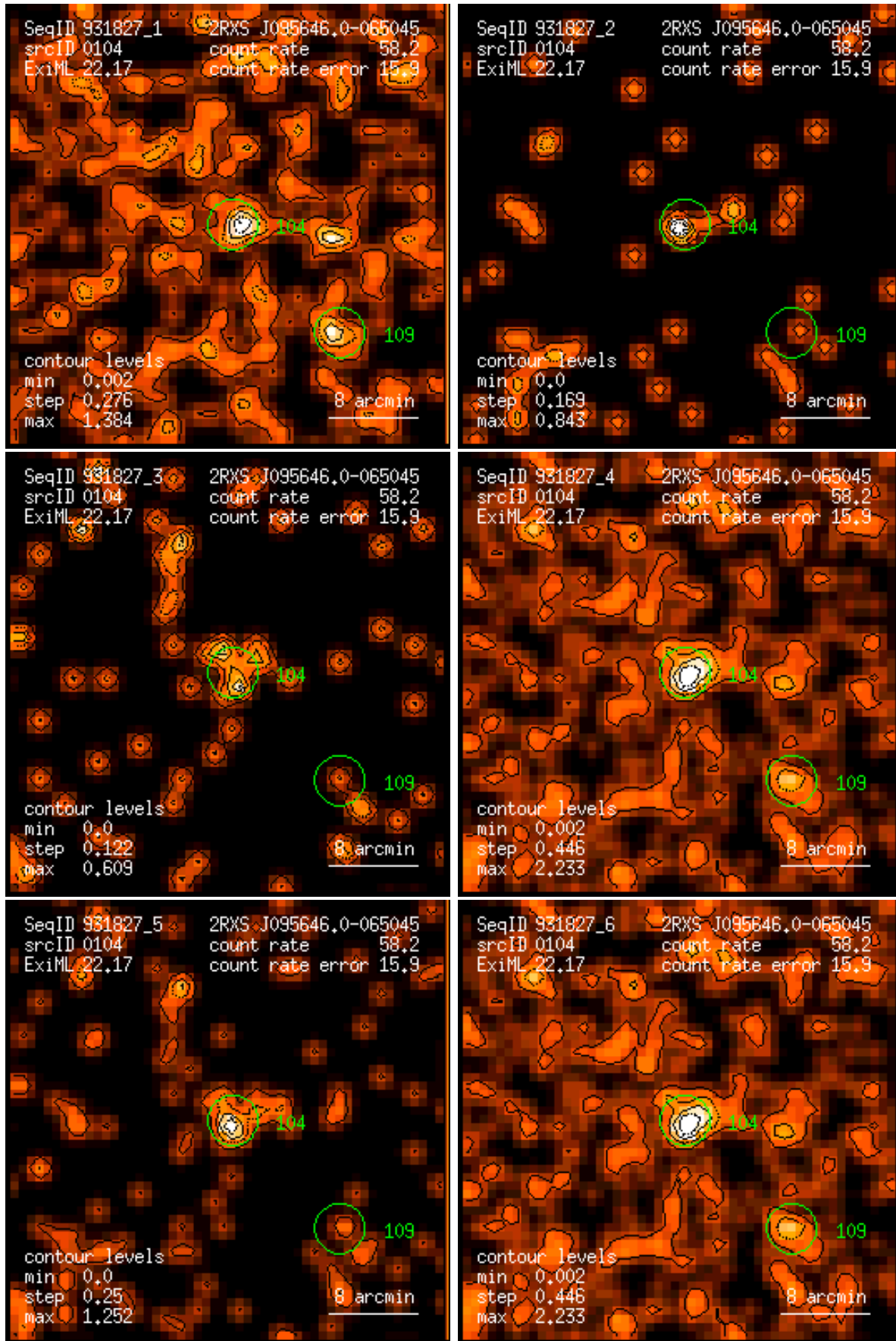
Figure 104: RASS 931827: detection 0104: band rate images, Gaussian filter: (1) PSPC channels 11 – 41, (2) 52 – 90, (3) 91 – 201, (4) 11 – 235, (5) 52 – 201, (6) 11 – 201. Broad band rates in counts/ks. Band rate contour levels in counts/ks/arcmin 2 .
