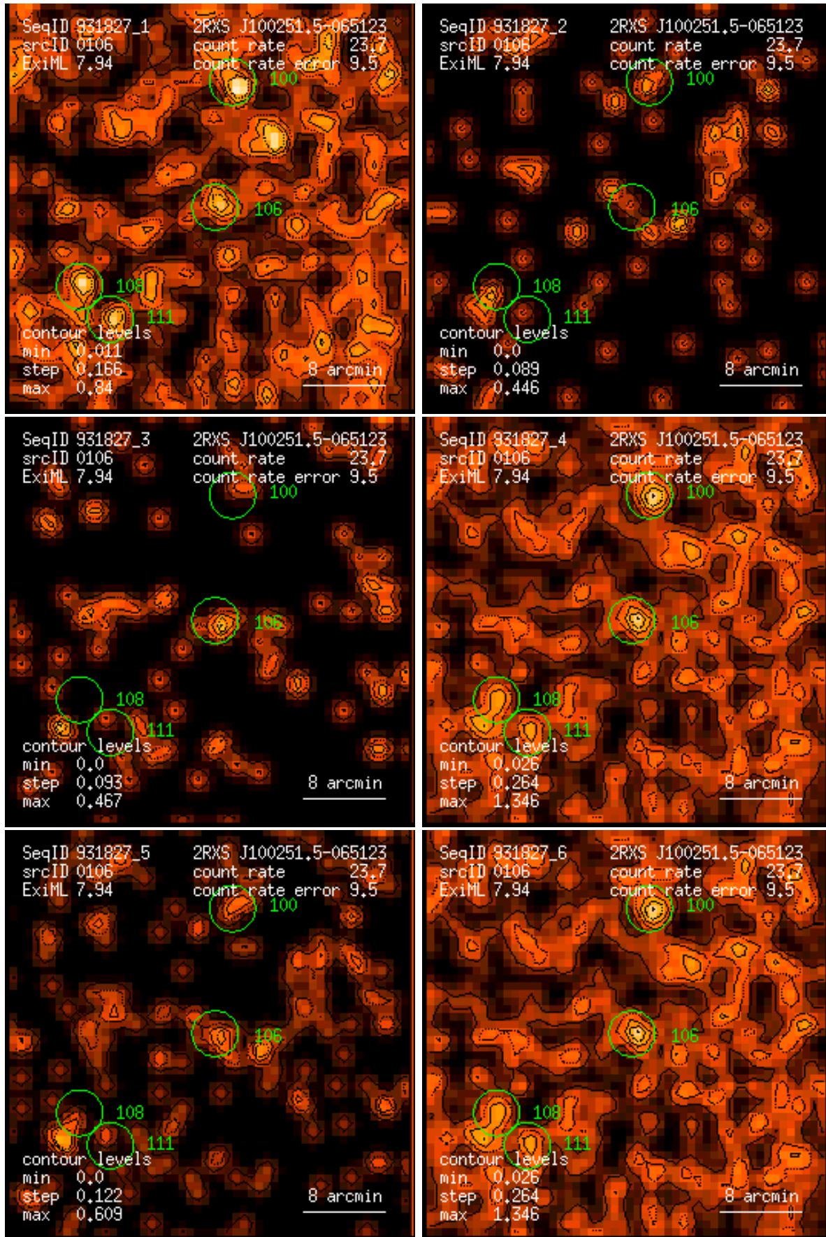
Figure 106: RASS 931827: detection 0106: band rate images, Gaussian filter: (1) PSPC channels 11 – 41, (2) 52 – 90, (3) 91 – 201, (4) 11 – 235, (5) 52 – 201, (6) 11 – 201. Broad band rates in counts/ks. Band rate contour levels in counts/ks/arcmin 2 .
