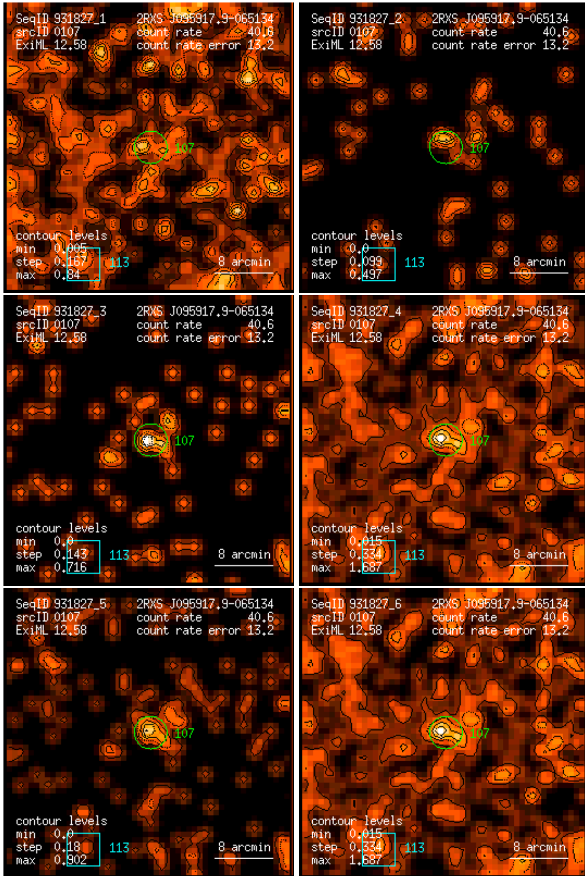
Figure 107: RASS 931827: detection 0107: band rate images, Gaussian filter: (1) PSPC channels 11 – 41, (2) 52 – 90, (3) 91 – 201, (4) 11 – 235, (5) 52 – 201, (6) 11 – 201. Broad band rates in counts/ks. Band rate contour levels in counts/ks/arcmin 2 .
