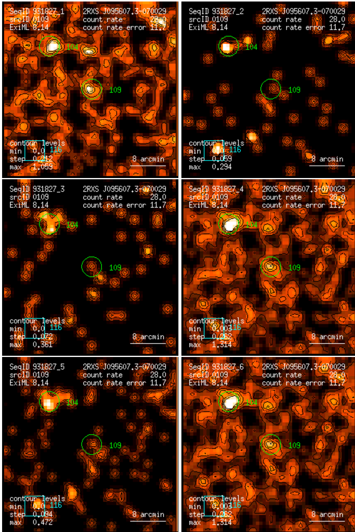
Figure 109: RASS 931827: detection 0109: band rate images, Gaussian filter: (1) PSPC channels 11 – 41, (2) 52 – 90, (3) 91 – 201, (4) 11 – 235, (5) 52 – 201, (6) 11 – 201. Broad band rates in counts/ks. Band rate contour levels in counts/ks/arcmin 2 .
