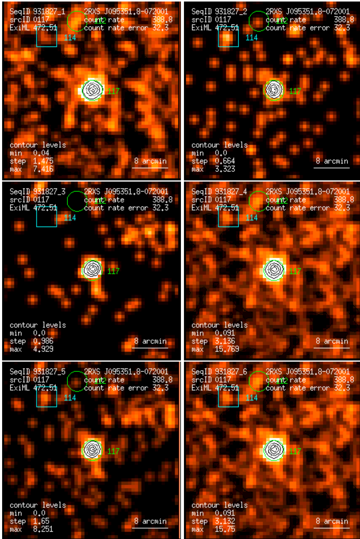
Figure 117: RASS 931827: detection 0117: band rate images, Gaussian filter: (1) PSPC channels 11 – 41, (2) 52 – 90, (3) 91 – 201, (4) 11 – 235, (5) 52 – 201, (6) 11 – 201. Broad band rates in counts/ks. Band rate contour levels in counts/ks/arcmin 2 .
