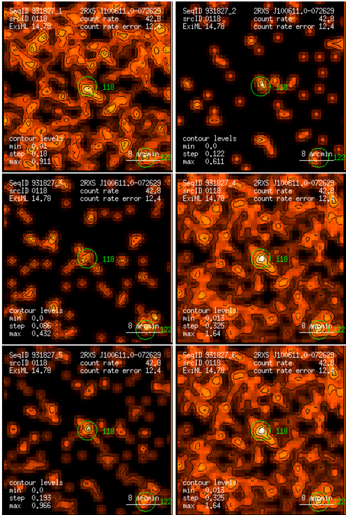
Figure 118: RASS 931827: detection 0118: band rate images, Gaussian filter: (1) PSPC channels 11 – 41, (2) 52 – 90, (3) 91 – 201, (4) 11 – 235, (5) 52 – 201, (6) 11 – 201. Broad band rates in counts/ks. Band rate contour levels in counts/ks/arcmin 2 .
