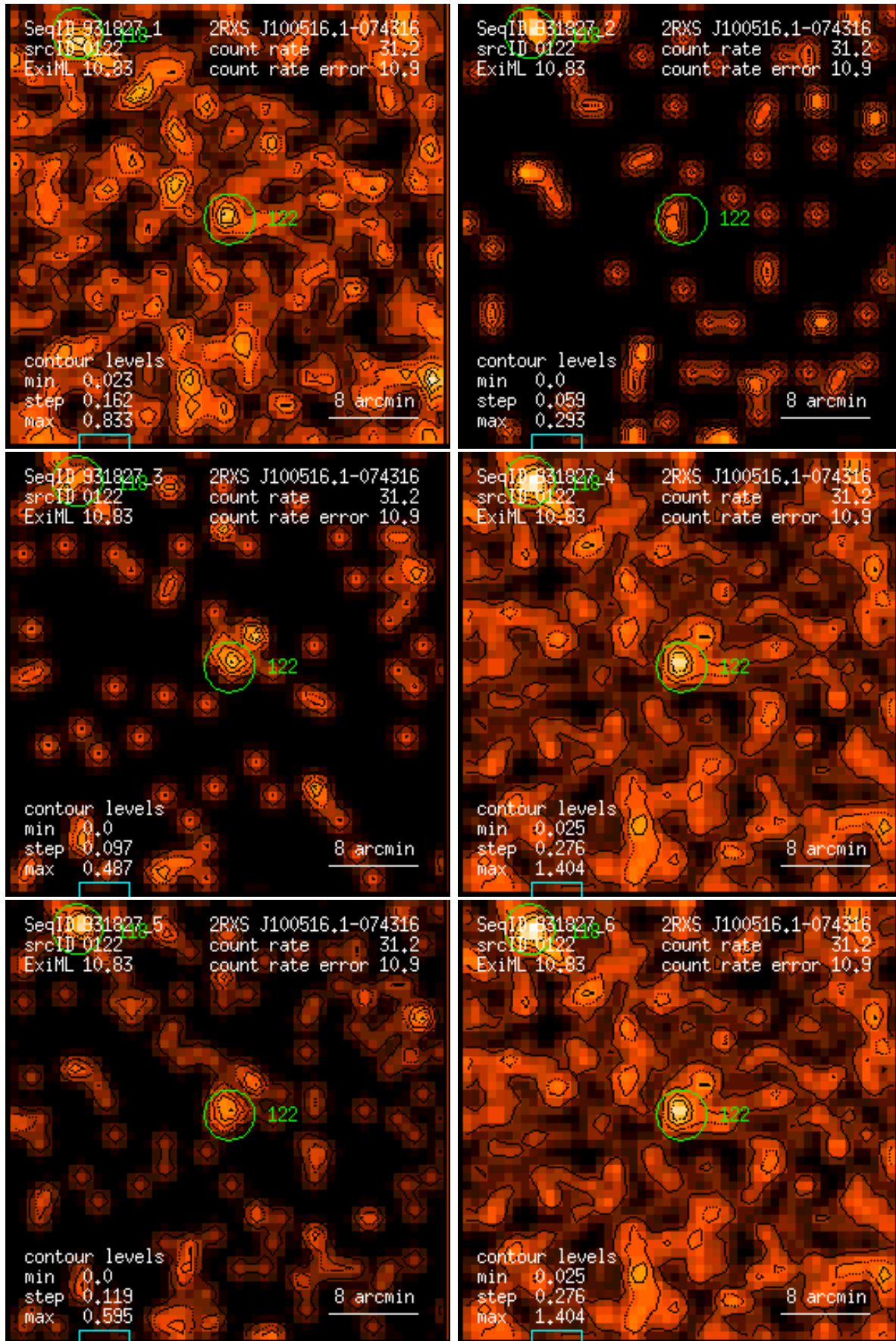
Figure 122: RASS 931827: detection 0122: band rate images, Gaussian filter: (1) PSPC channels 11 – 41, (2) 52 – 90, (3) 91 – 201, (4) 11 – 235, (5) 52 – 201, (6) 11 – 201. Broad band rates in counts/ks. Band rate contour levels in counts/ks/arcmin 2 .
