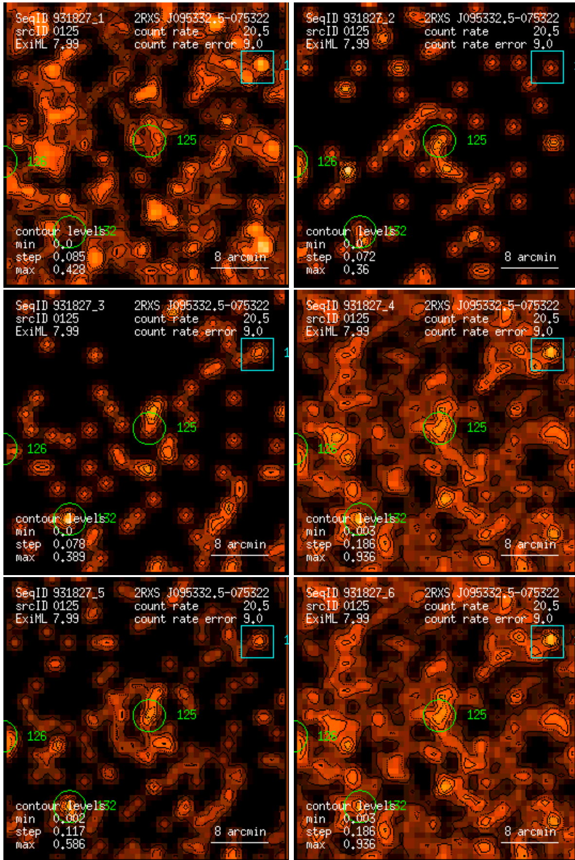
Figure 125: RASS 931827: detection 0125: band rate images, Gaussian filter: (1) PSPC channels 11 – 41, (2) 52 – 90, (3) 91 – 201, (4) 11 – 235, (5) 52 – 201, (6) 11 – 201. Broad band rates in counts/ks. Band rate contour levels in counts/ks/arcmin 2 .
