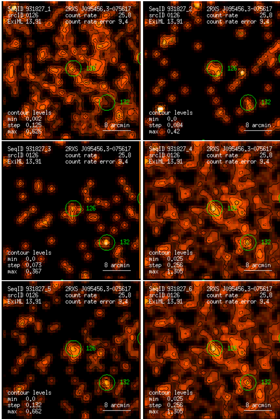
Figure 126: RASS 931827: detection 0126: band rate images, Gaussian filter: (1) PSPC channels 11 – 41, (2) 52 – 90, (3) 91 – 201, (4) 11 – 235, (5) 52 – 201, (6) 11 – 201. Broad band rates in counts/ks. Band rate contour levels in counts/ks/arcmin 2 .
