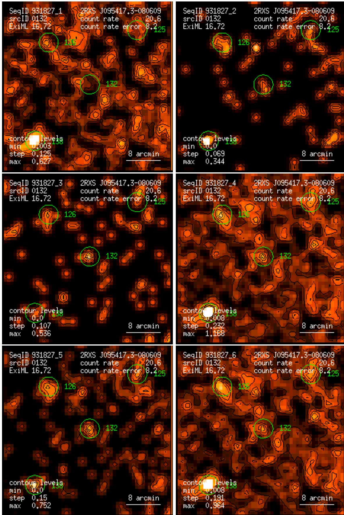
Figure 132: RASS 931827: detection 0132: band rate images, Gaussian filter: (1) PSPC channels 11 – 41, (2) 52 – 90, (3) 91 – 201, (4) 11 – 235, (5) 52 – 201, (6) 11 – 201. Broad band rates in counts/ks. Band rate contour levels in counts/ks/arcmin 2 .
