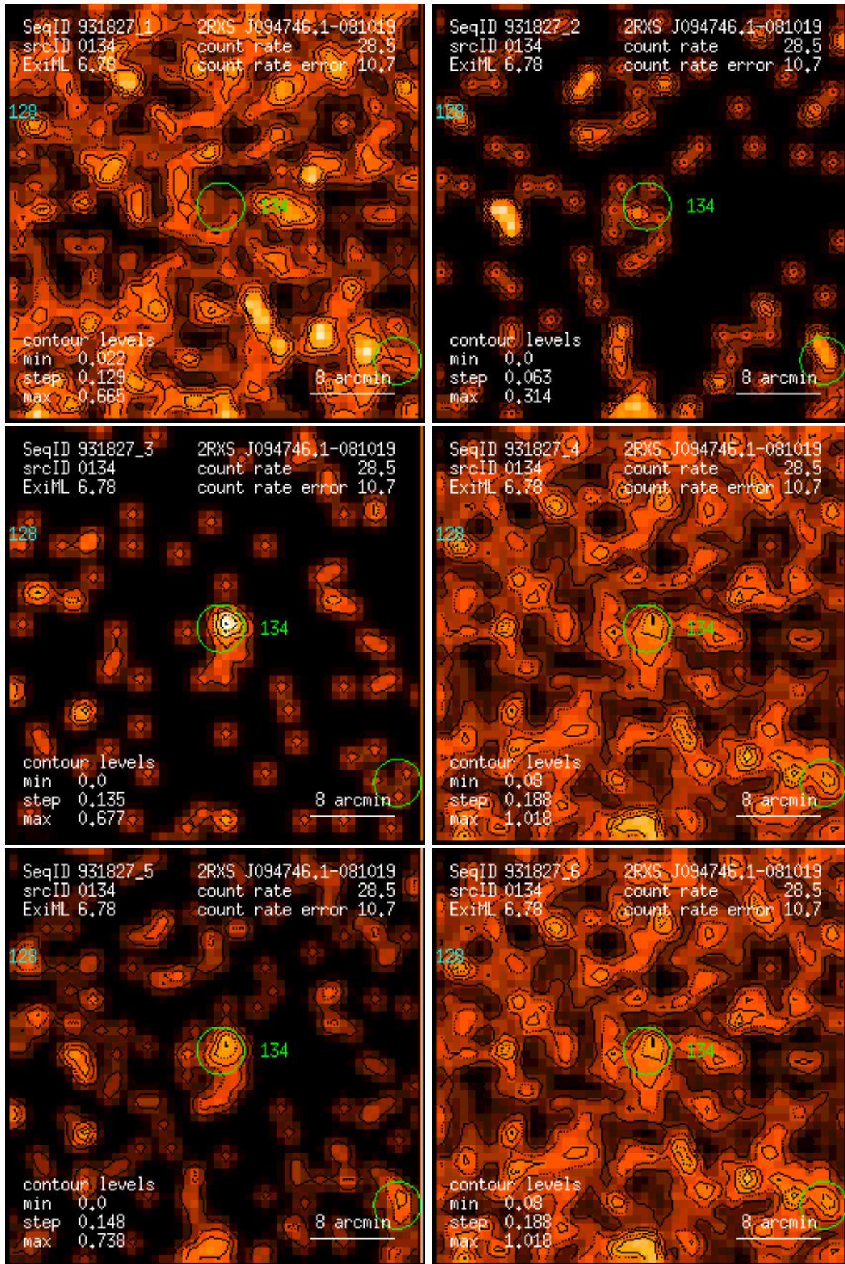
Figure 134: RASS 931827: detection 0134: band rate images, Gaussian filter: (1) PSPC channels 11 – 41, (2) 52 – 90, (3) 91 – 201, (4) 11 – 235, (5) 52 – 201, (6) 11 – 201. Broad band rates in counts/ks. Band rate contour levels in counts/ks/arcmin 2 .
