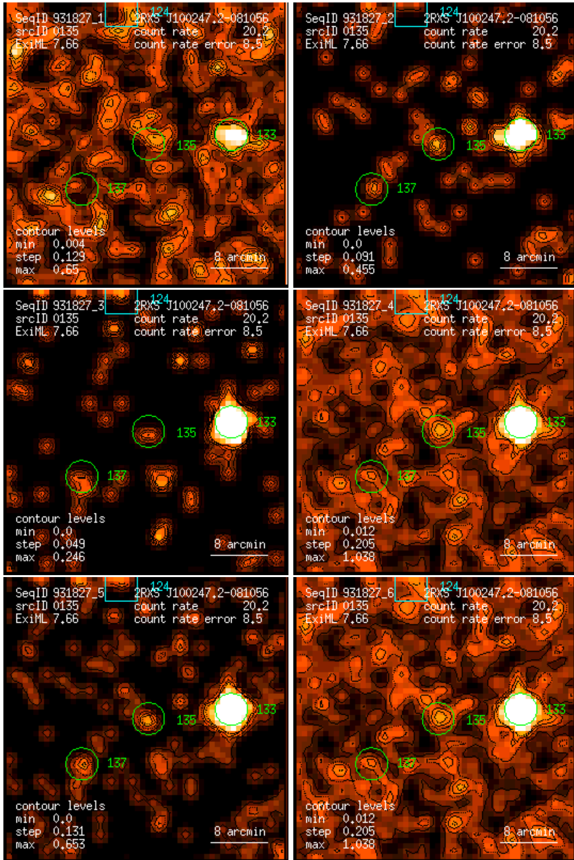
Figure 135: RASS 931827: detection 0135: band rate images, Gaussian filter: (1) PSPC channels 11 – 41, (2) 52 – 90, (3) 91 – 201, (4) 11 – 235, (5) 52 – 201, (6) 11 – 201. Broad band rates in counts/ks. Band rate contour levels in counts/ks/arcmin 2 .
