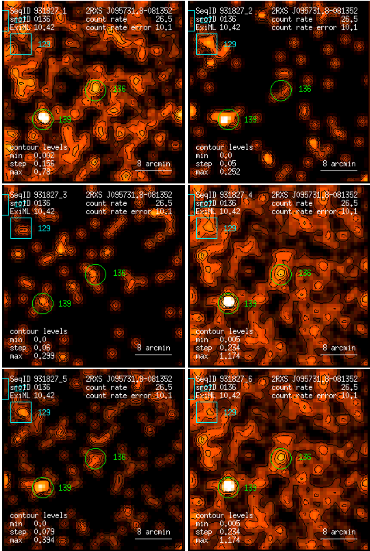
Figure 136: RASS 931827: detection 0136: band rate images, Gaussian filter: (1) PSPC channels 11 – 41, (2) 52 – 90, (3) 91 – 201, (4) 11 – 235, (5) 52 – 201, (6) 11 – 201. Broad band rates in counts/ks. Band rate contour levels in counts/ks/arcmin 2 .
