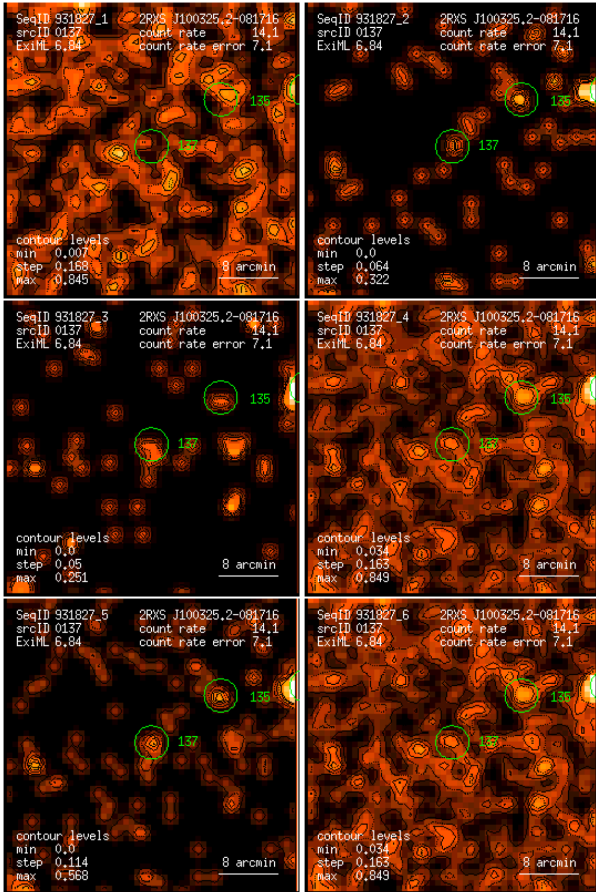
Figure 137: RASS 931827: detection 0137: band rate images, Gaussian filter: (1) PSPC channels 11 – 41, (2) 52 – 90, (3) 91 – 201, (4) 11 – 235, (5) 52 – 201, (6) 11 – 201. Broad band rates in counts/ks. Band rate contour levels in counts/ks/arcmin 2 .
