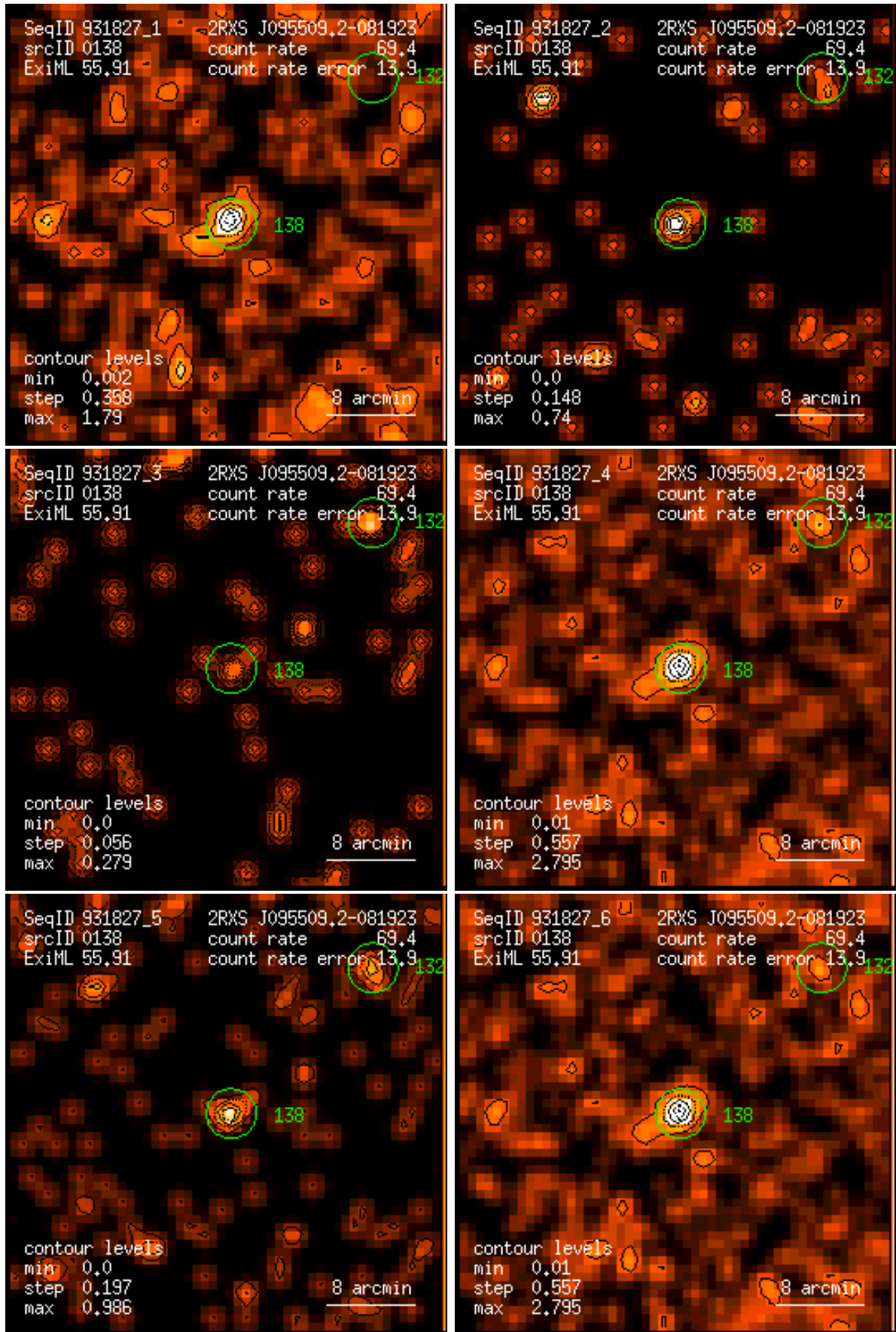
Figure 138: RASS 931827: detection 0138: band rate images, Gaussian filter: (1) PSPC channels 11 – 41, (2) 52 – 90, (3) 91 – 201, (4) 11 – 235, (5) 52 – 201, (6) 11 – 201. Broad band rates in counts/ks. Band rate contour levels in counts/ks/arcmin 2 .
