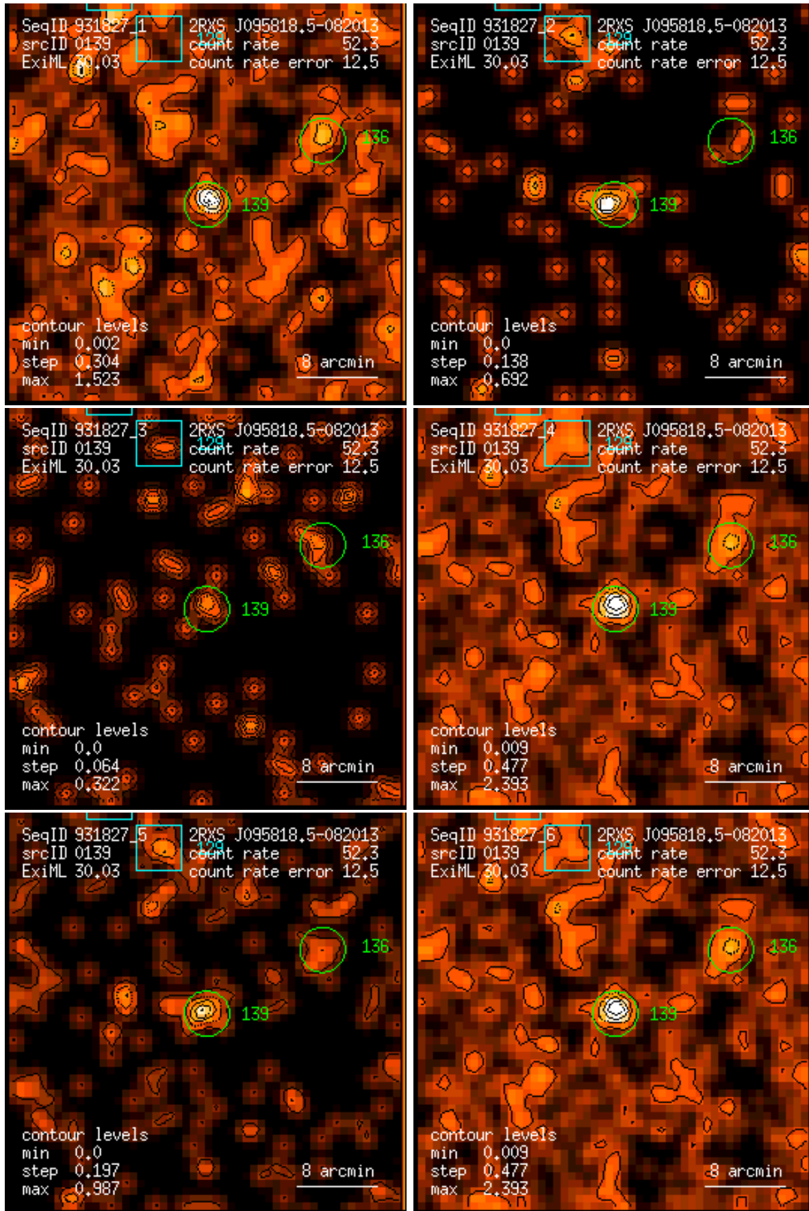
Figure 139: RASS 931827: detection 0139: band rate images, Gaussian filter: (1) PSPC channels 11 – 41, (2) 52 – 90, (3) 91 – 201, (4) 11 – 235, (5) 52 – 201, (6) 11 – 201. Broad band rates in counts/ks. Band rate contour levels in counts/ks/arcmin 2 .
