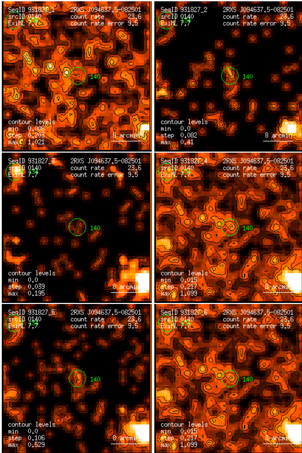
Figure 140: RASS 931827: detection 0140: band rate images, Gaussian filter: (1) PSPC channels 11 – 41, (2) 52 – 90, (3) 91 – 201, (4) 11 – 235, (5) 52 – 201, (6) 11 – 201. Broad band rates in counts/ks. Band rate contour levels in counts/ks/arcmin 2 .
