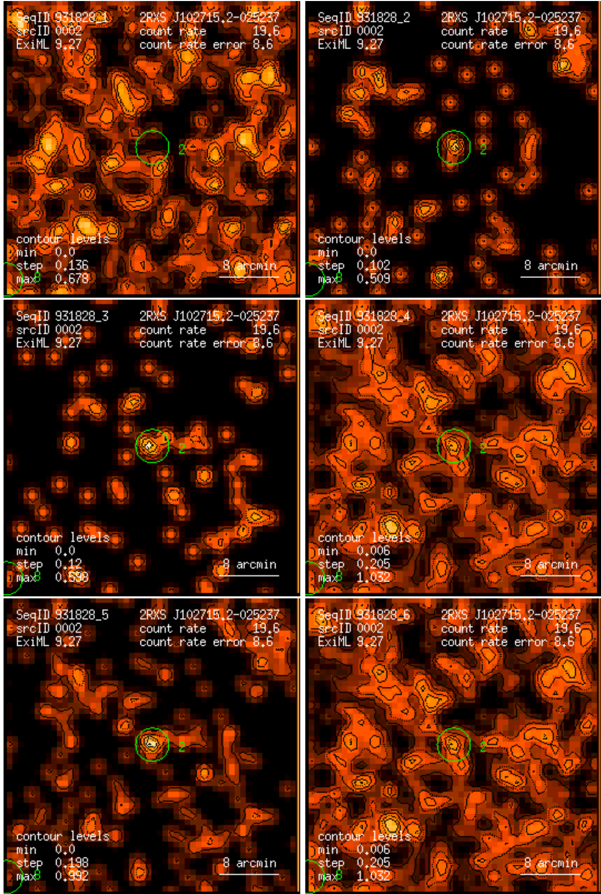
Figure 2: RASS 931828: detection 0002: band rate images, Gaussian filter: (1) PSPC channels 11 – 41, (2) 52 – 90, (3) 91 – 201, (4) 11 – 235, (5) 52 – 201, (6) 11 – 201. Broad band rates in counts/ks. Band rate contour levels in counts/ks/arcmin 2 .
