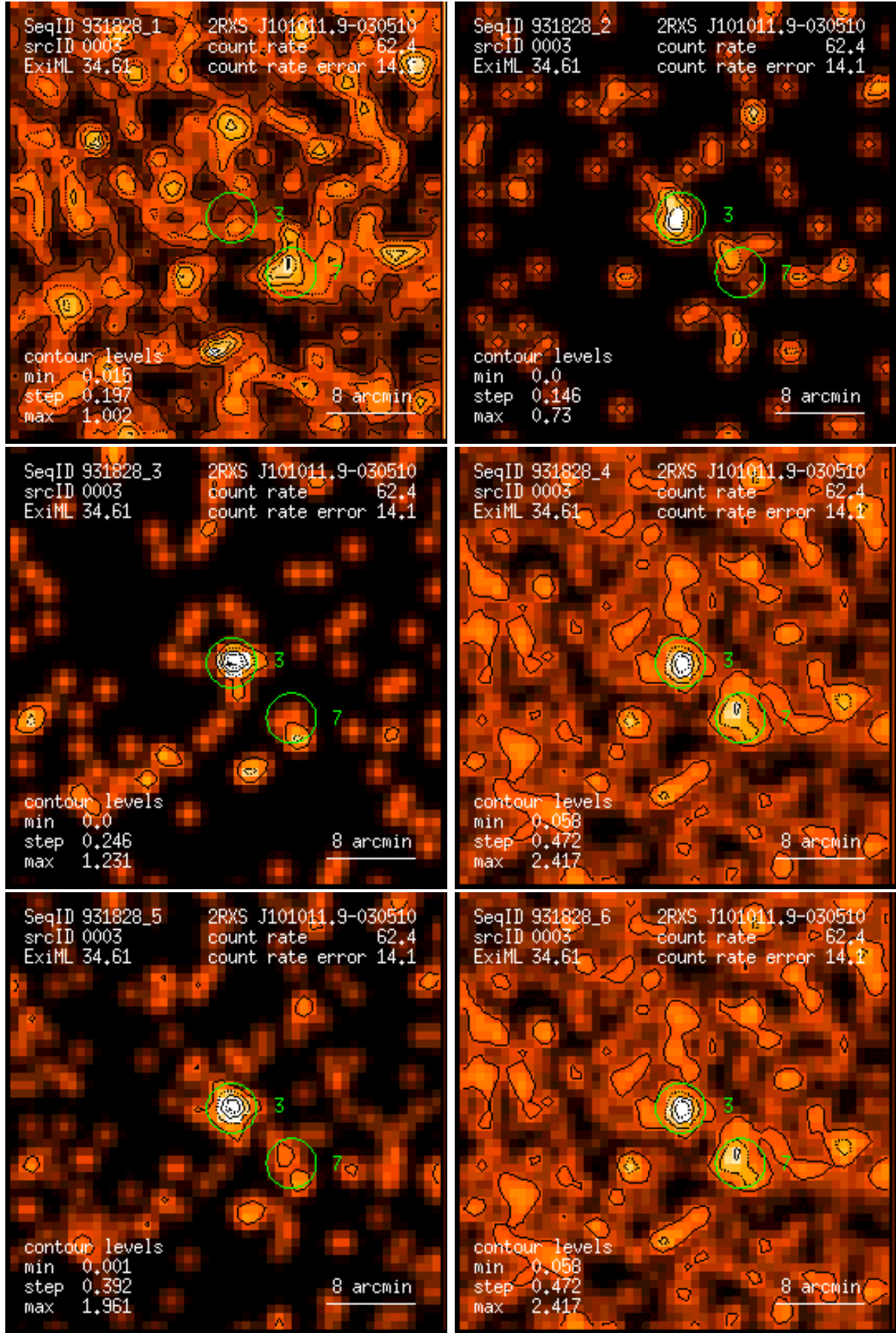
Figure 3: RASS 931828: detection 0003: band rate images, Gaussian filter: (1) PSPC channels 11 – 41, (2) 52 – 90, (3) 91 – 201, (4) 11 – 235, (5) 52 – 201, (6) 11 – 201. Broad band rates in counts/ks. Band rate contour levels in counts/ks/arcmin 2 .
