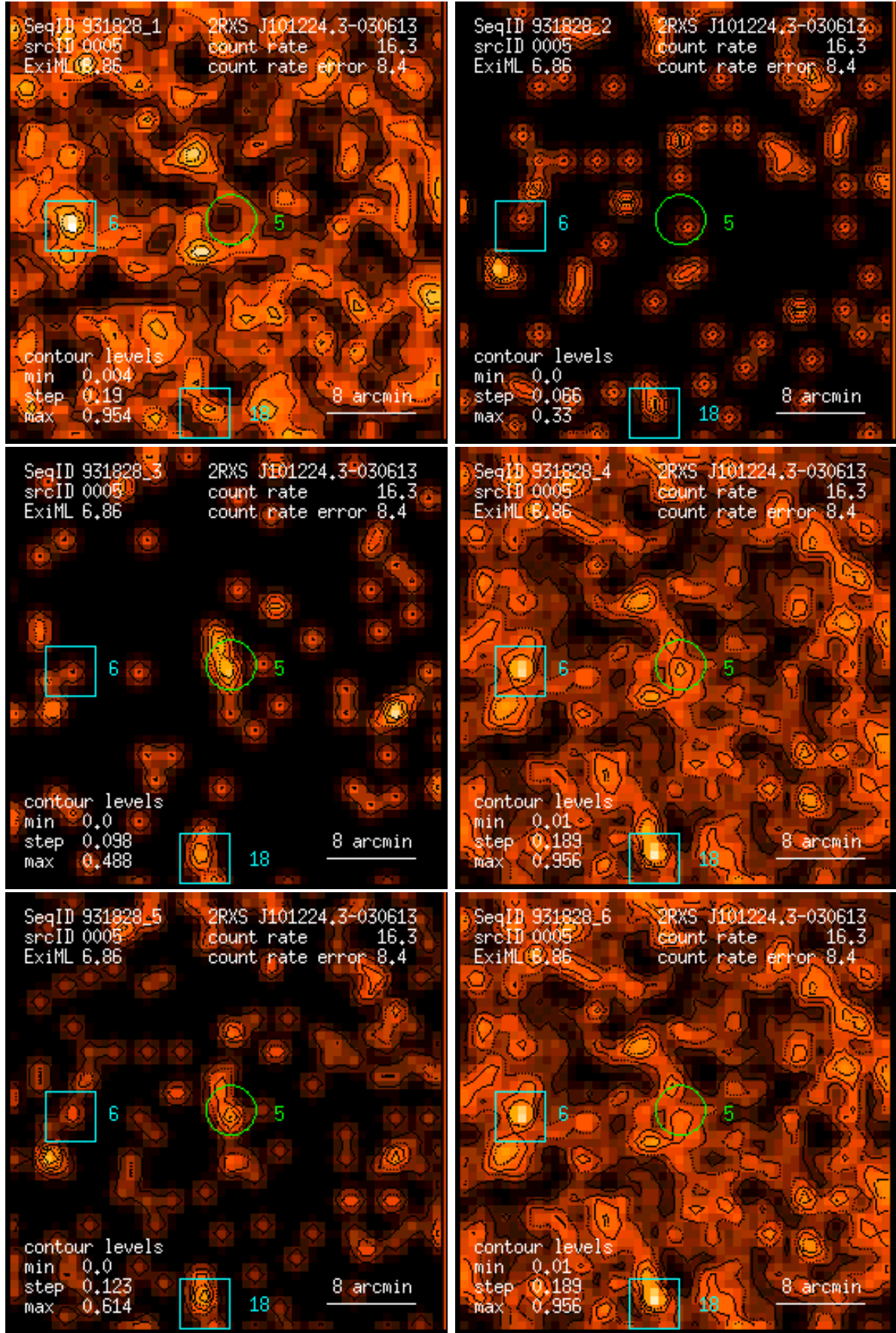
Figure 5: RASS 931828: detection 0005: band rate images, Gaussian filter: (1) PSPC channels 11 – 41, (2) 52 – 90, (3) 91 – 201, (4) 11 – 235, (5) 52 – 201, (6) 11 – 201. Broad band rates in counts/ks. Band rate contour levels in counts/ks/arcmin 2 .
