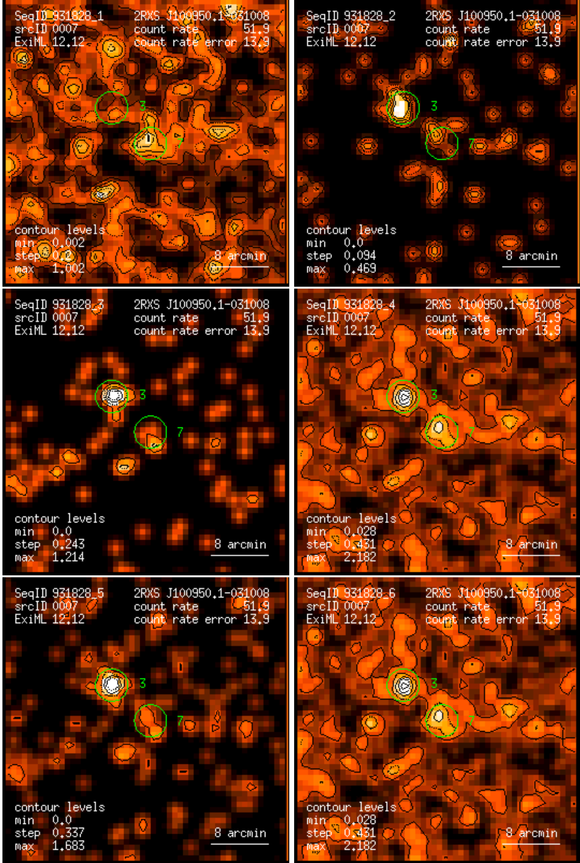
Figure 7: RASS 931828: detection 0007: band rate images, Gaussian filter: (1) PSPC channels 11 – 41, (2) 52 – 90, (3) 91 – 201, (4) 11 – 235, (5) 52 – 201, (6) 11 – 201. Broad band rates in counts/ks. Band rate contour levels in counts/ks/arcmin 2 .
