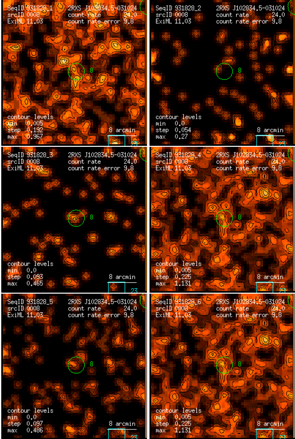
Figure 8: RASS 931828: detection 0008: band rate images, Gaussian filter: (1) PSPC channels 11 – 41, (2) 52 – 90, (3) 91 – 201, (4) 11 – 235, (5) 52 – 201, (6) 11 – 201. Broad band rates in counts/ks. Band rate contour levels in counts/ks/arcmin 2 .
